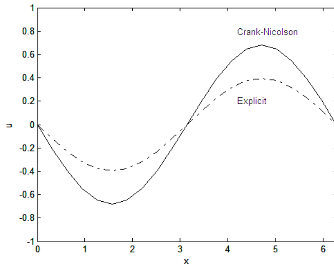
Figure (1) Comparison of explicit and Crank-Nicolson methods
