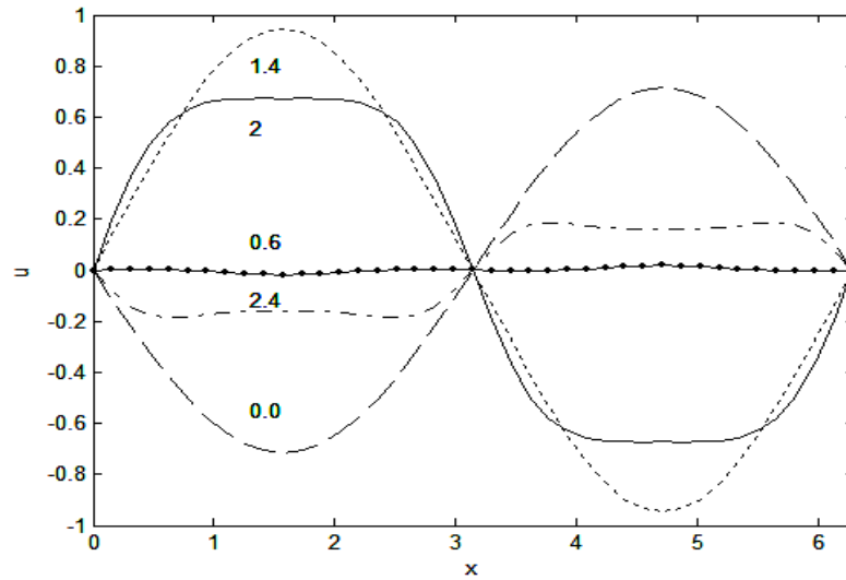
Figure (7) Explicit method with different \varepsilon , \varepsilon = 0.0, \varepsilon = 0.6, \varepsilon = 1.4, \varepsilon = 2, \varepsilon = 2.4
