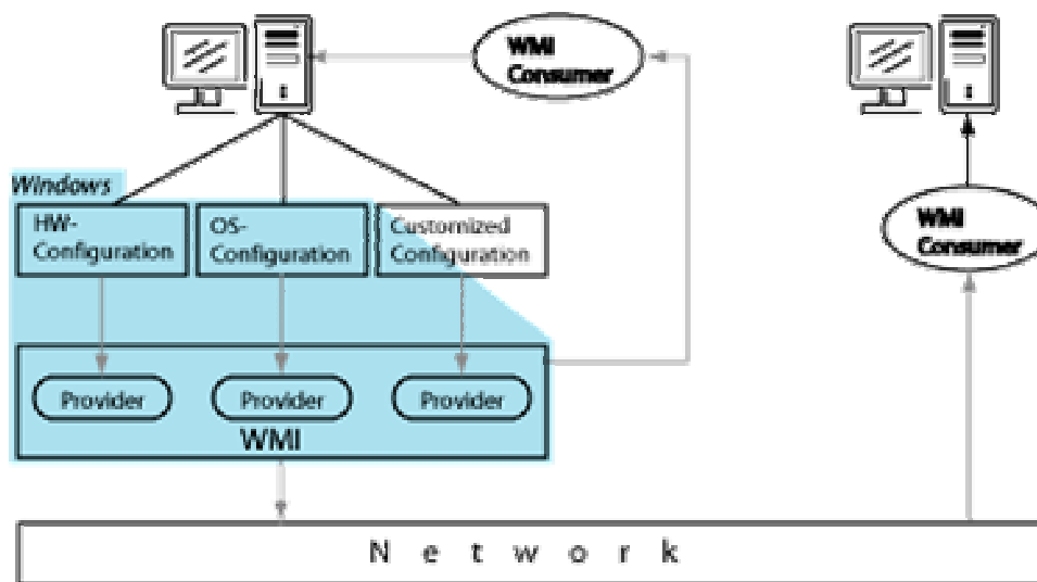
Figure (3): WMI architecture
