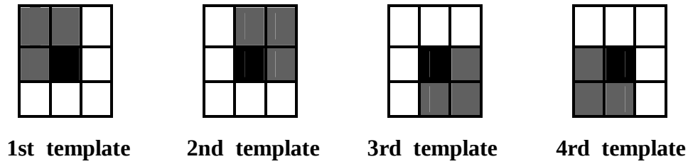
Figure (5): 4 Basic templates used in the proposed algorithm, the central ( black ) pixels only will be flipped from “0” to “1” or vice versa.
