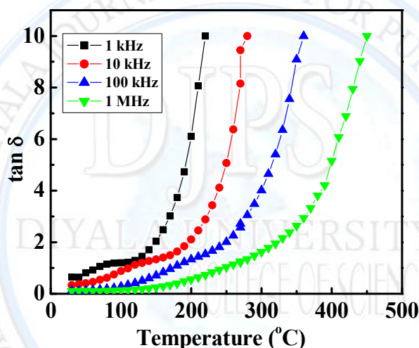
Fig. 6 Variation of the dielectric loss with temperature for 0.30\text{Ni}_{0.7}\text{Zn}_{0.3}\text{Fe}_2\text{O}_4 + 0.70\text{ PLZT} composite annealed at 1100^\circ\text{C} .
