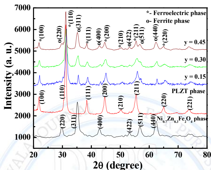
Fig. 1. XRD patterns of (y)\text{Ni}_{0.7}\text{Zn}_{0.3}\text{Fe}_2\text{O}_4 + (1-y)\text{ PLZT} composites where y = 0.00, 0.15, 0.30, 0.45 and 1 sintered at 700^\circ\text{C} .
