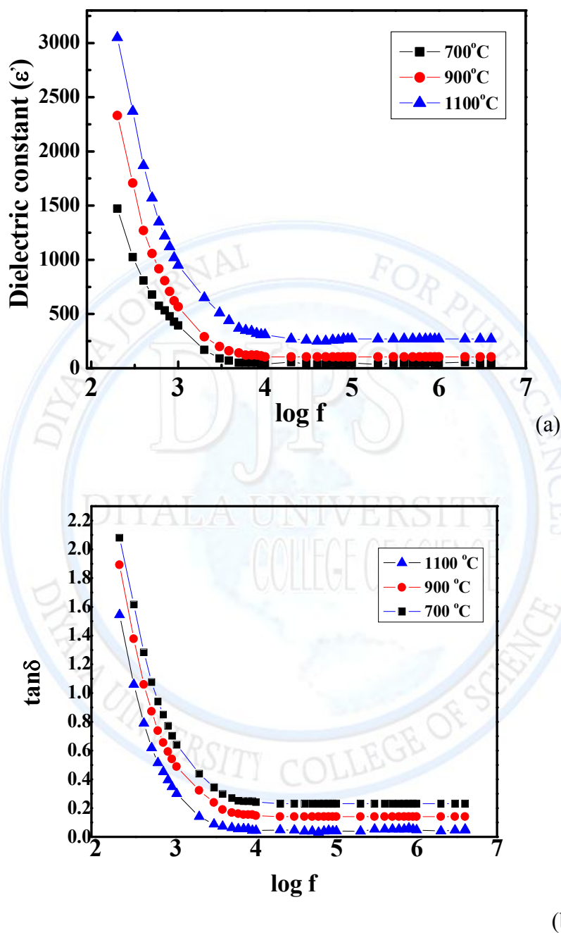
Fig.4 Variation of the (a) dielectric constant and (b) dielectric loss with frequency for 0.30\text{Ni}_{0.7}\text{Zn}_{0.3}\text{Fe}_2\text{O}_4 + 0.70\text{PLZT} composite annealed at different temperatures.
