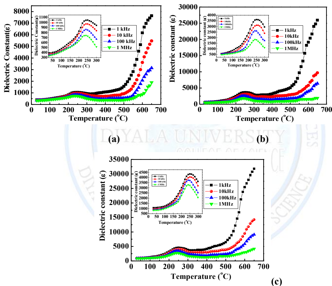
Fig.5 (a-c) Variation of the dielectric constant with temperature for 0.30\text{Ni}_{0.7}\text{Zn}_{0.3}\text{Fe}_2\text{O}_4 + 0.70\text{PLZT} composite annealed at different temperatures (a) 700 °C, (b) 900 °C and (c) 1100 °C
