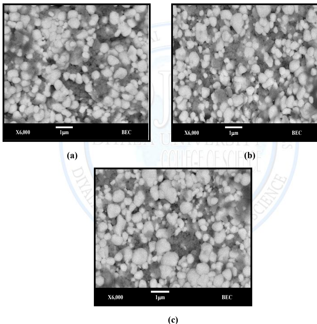
Fig. 3 SEM micrograph of 0.30\text{Ni}_{0.7}\text{Zn}_{0.3}\text{Fe}_2\text{O}_4 + 0.70 \text{ PLZT} composite annealed at different temperatures (a) 700 °C, (b) 900 °C and ( c ) 1100 °C.
