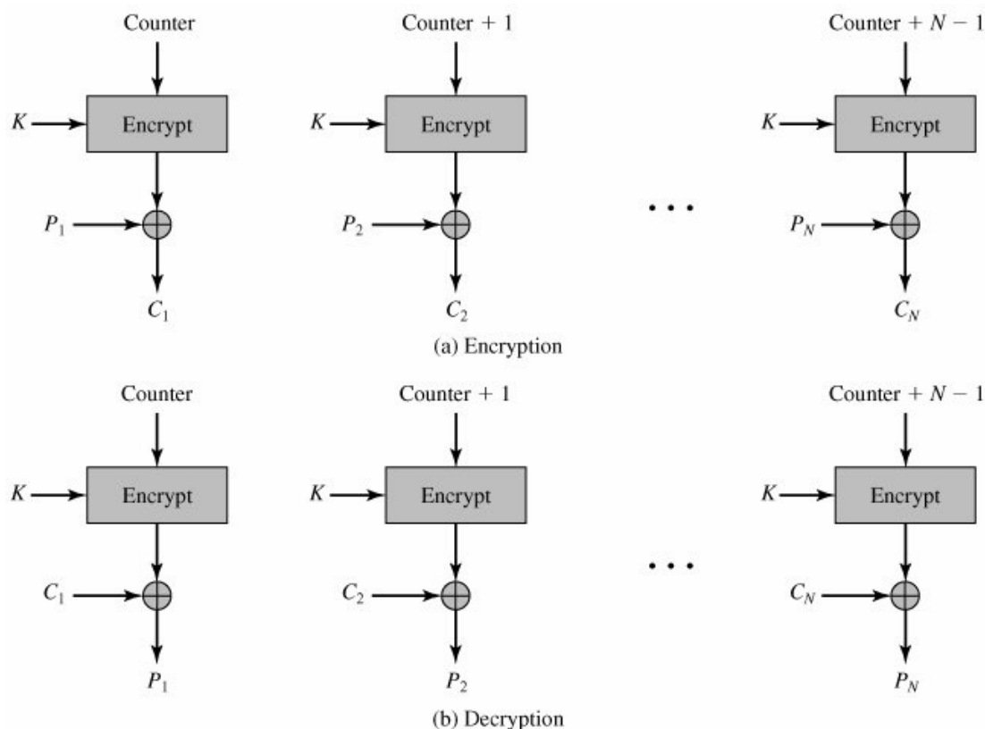
Fig.1: Counter Mode
