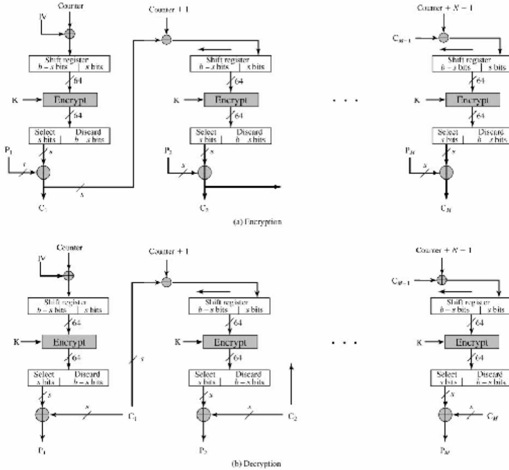
Fig.3: s-bit Counter Cipher Feedback (CCFB) Mode
