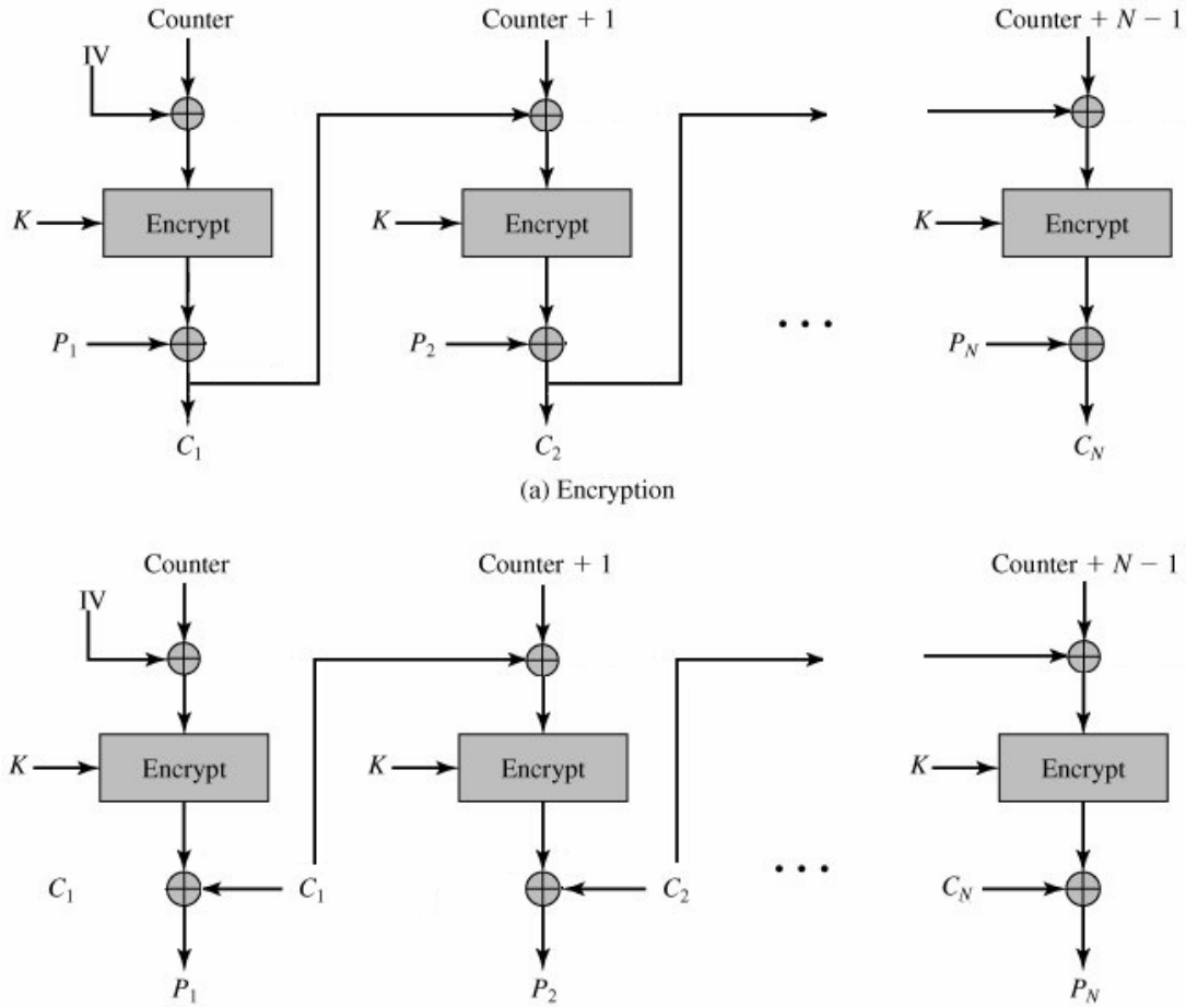
Fig.2: Counter Cipher Block Chaining (CCBC) Mode
