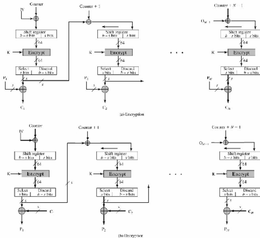
Fig.4: s-bit Counter Output Feedback (COFB) Mode
