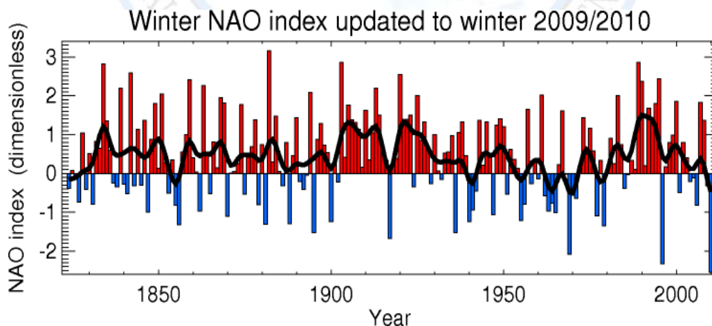
Fig. 1: The time series plot of NAO index for winter (Dec-Mar) based on normalized sea level pressure between Gibraltar and Iceland for the period (1823-2009) [8] .
