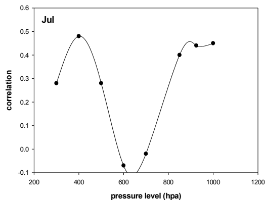
Fig. 8: Correlation coefficient of specific humidity with NAOI as a function of pressure level at Jul
