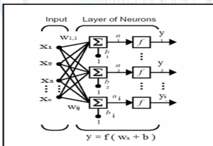
Figure 1. Multi-Layer Perceptron's Architecture.
