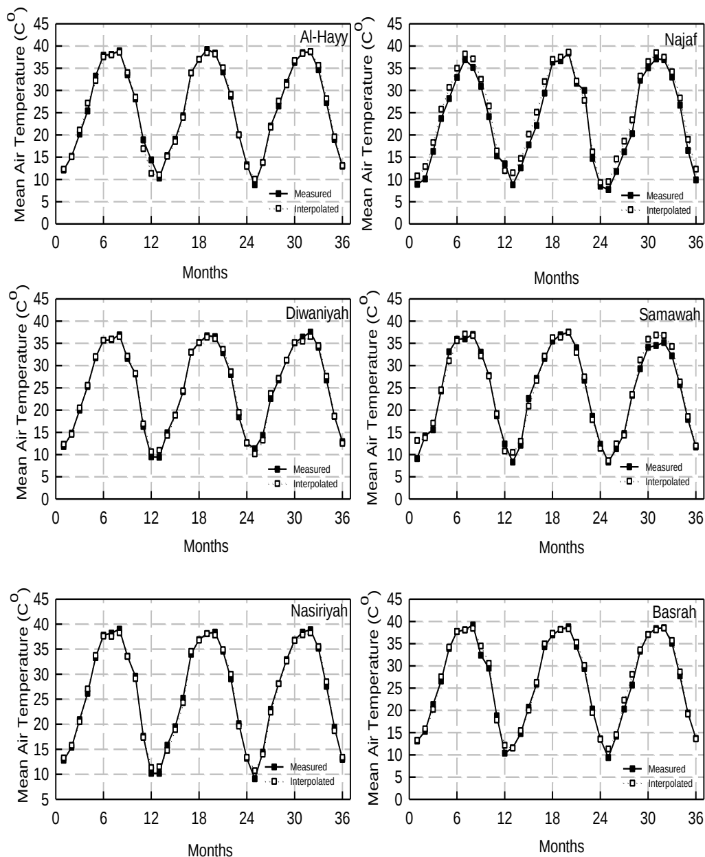
Figure 5. Represents the measured and interpolated monthly mean air temperature for Stations Al-Hayy, Najaf, Diwaniyah, Samawah, Nasiriyah and Basrah.
