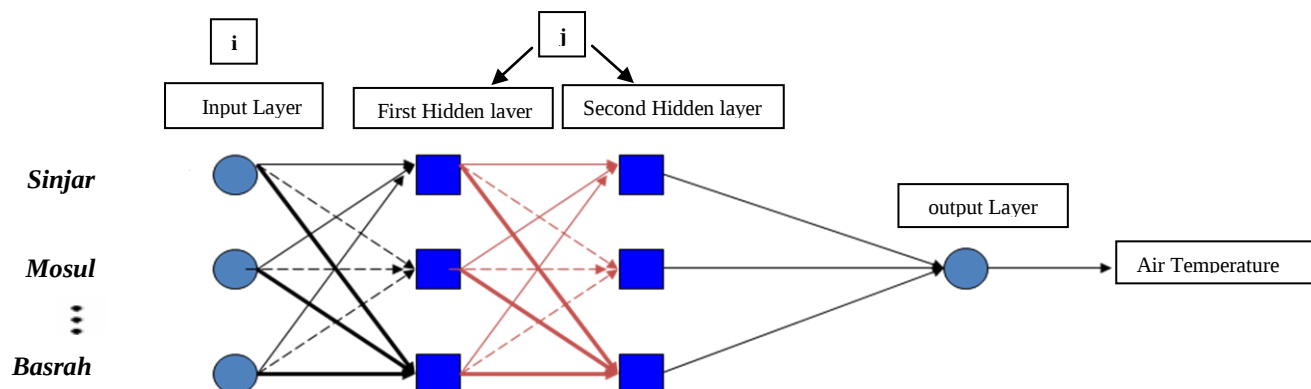
Figure 2. (ANN) architecture used in the interpolation process.
