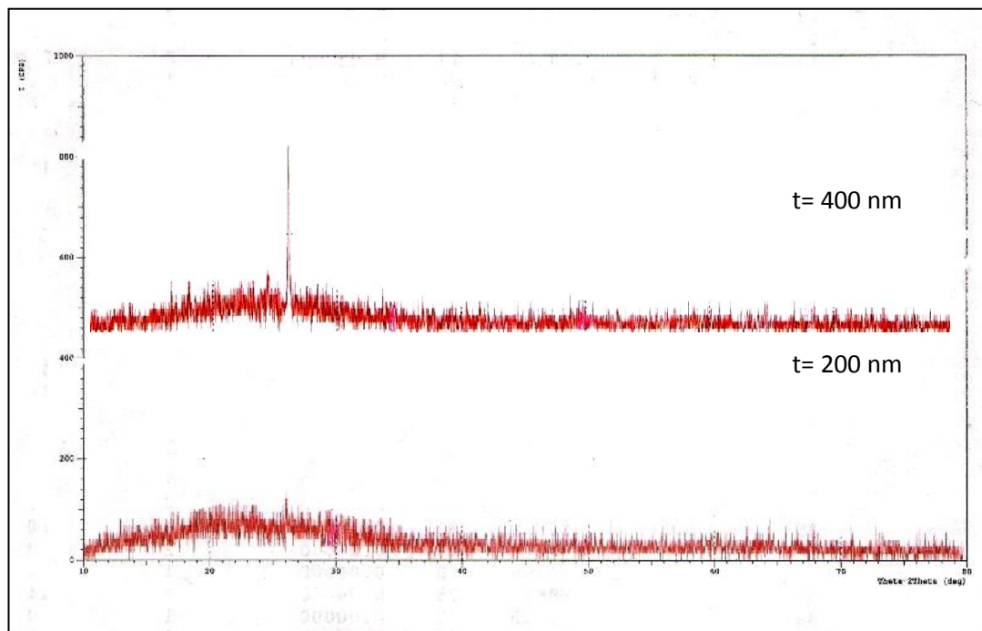
Figure 2. X-Ray diffractograms of CdS films with different thicknesses
