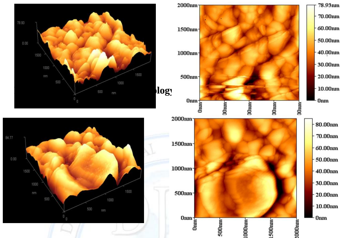
Figure (3b). AFM images morphology of CdS film at the thickness (400 nm).
