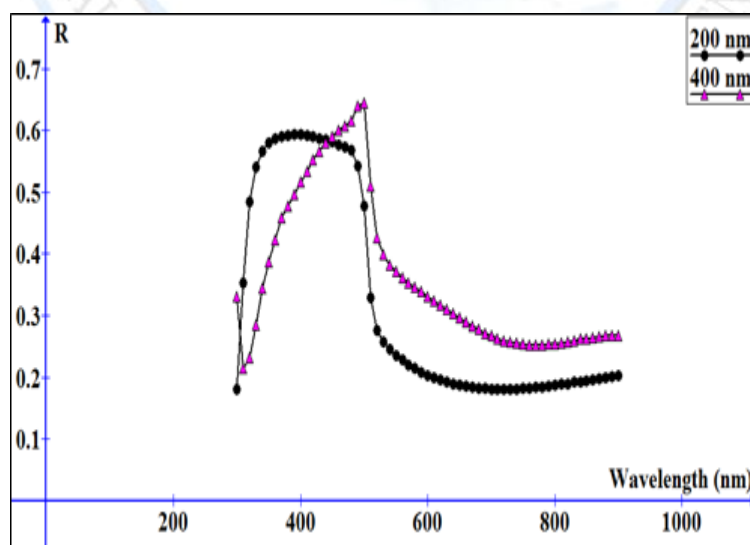
Figure 4. Reflectance Spectra of CdS thin films as a function of wavelength
