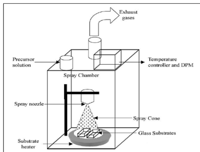
Figure 1. Spray pyrolysis set-up used for thin film preparation.
