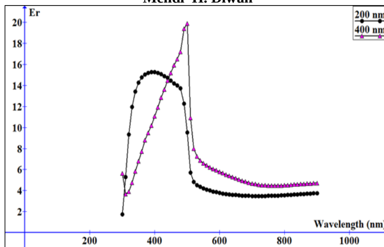
Figure 6. Real part of dielectric constant( E_r ) of CdS thin films as a functions of wavelength
