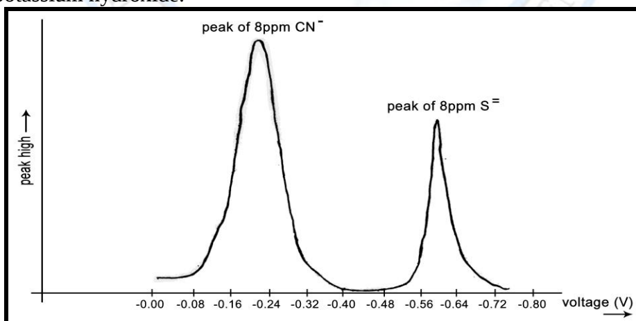
Figure 3 polarogram of cyanide and sulfide ions in support (boric acid + KOH) using Dp mode using differential puls polarography. Interfering ions \text{Cl}^- , \text{Ca}^{2+} , \text{Mg}^{2+} , \text{Fe}^{3+} and \text{Cu}^{2+} on Cyanide and sulfide determination by polarography was studied.
