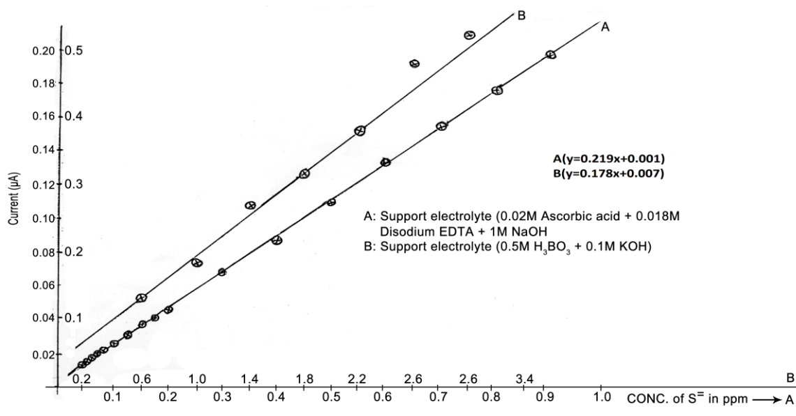
Figure 2 Calibration curve of sulfide ion by polarographic method using two supporting electrolytes.
