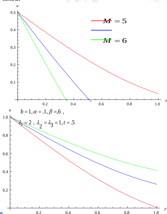
Fig.(5) Velocity u(y,t) versus y for different value of M when the other parameters are fixed.
