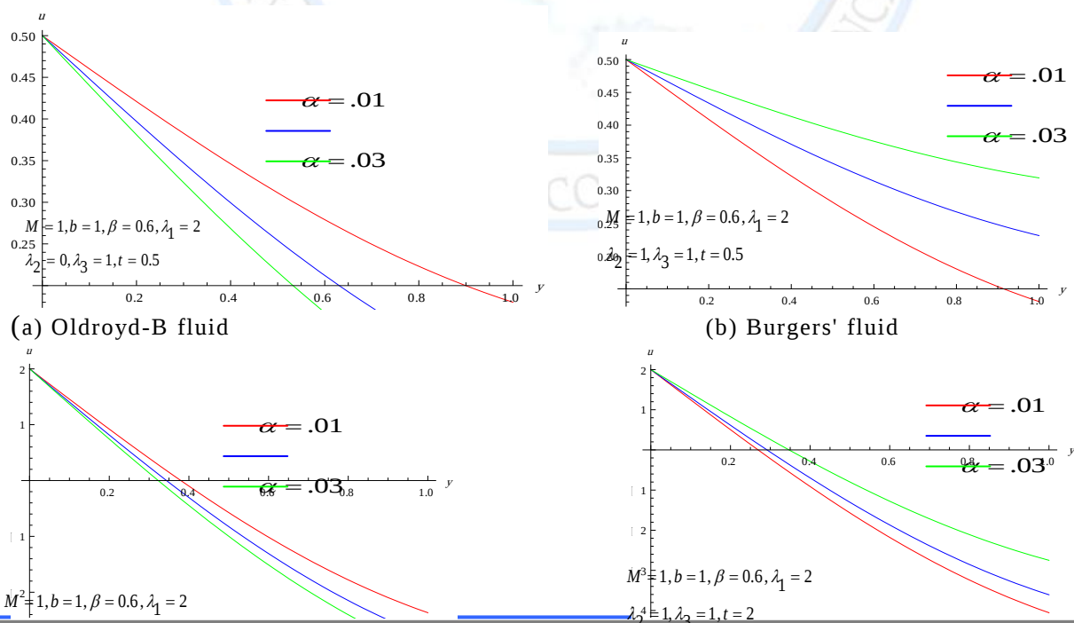
Fig.(1) Velocity u(y,t) versus y for different value of \alpha when the other parameters are fixed.
