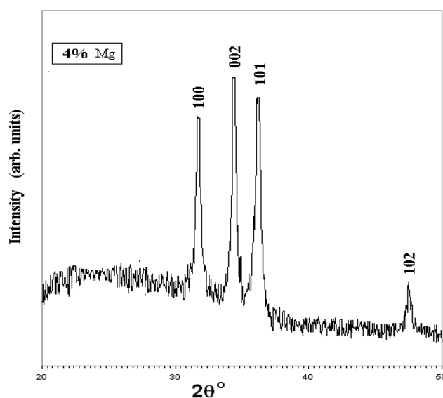
Figure (3): XRD pattern for ZnO: 4% Mg.
