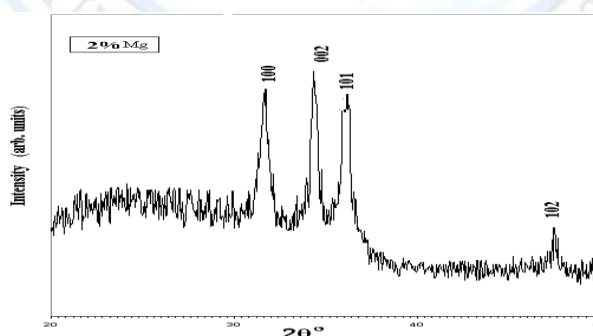
Figure (2): XRD pattern for ZnO: 2% Mg.
