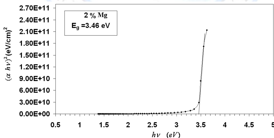
Figure (6): Direct transition as a function of photon energy for ZnO: Mg
