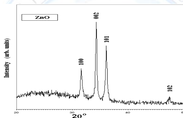
Figure (1): XRD pattern for undoped ZnO
