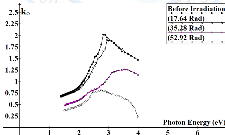
Figure (6) Extinction coefficient as a function of photon energy.
