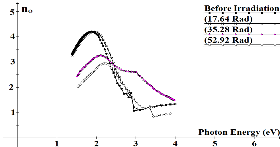
Figure (5) Refractive index as a function of Photon energy.
