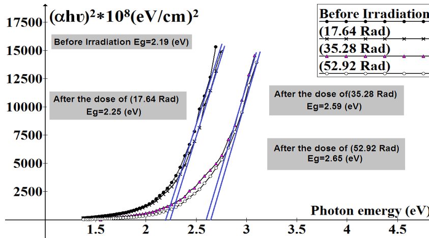
Figure. (4): Optical band gap E_g estimation for (\text{Mn}_2\text{O}_3)_{1-x}(\text{CuO})_x films before and after irradiation
