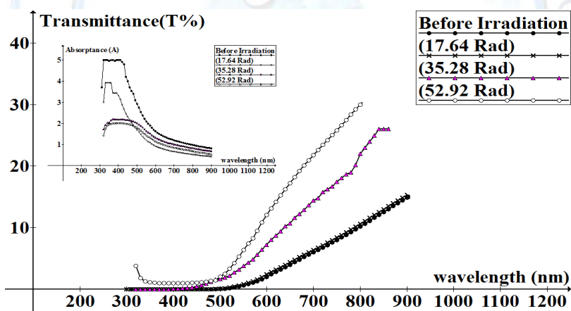
Figure (1) Optical transmittance as a function of wavelength.
