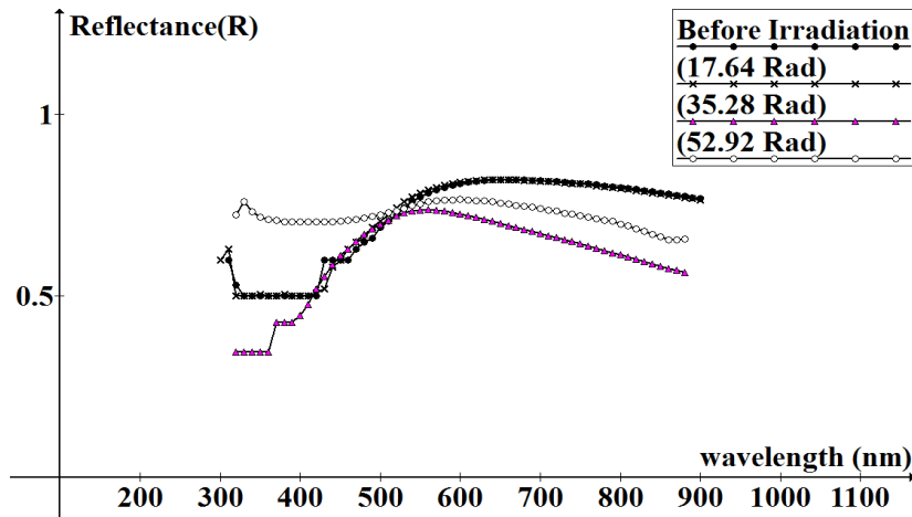
Figure (2) Reflectance as a function of wavelength.
