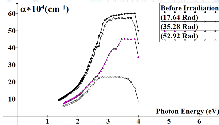
Figure (3) Absorption coefficient as a function of Photon energy.
