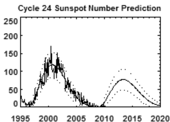
Figure 4: Monthly averaged sunspot number as a function of time
