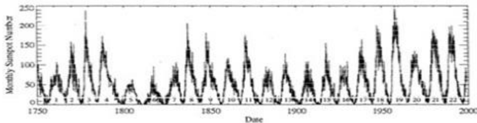
Figure 1: Monthly averaged International Sunspot Number as a function of time. The
