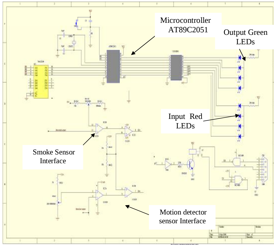
Fig.(3 ) The Schematic Diagram of Board 2
