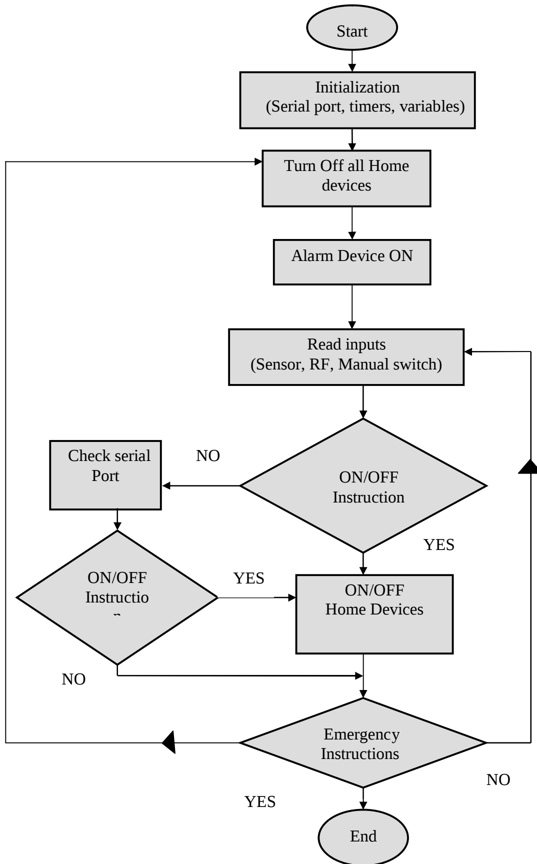
Fig.(7) Programming Microcontroller With Protection System Flow Chart
