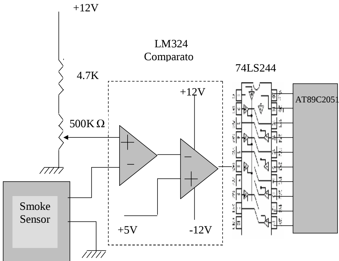
Fig.(5) Block Diagram of Interface Smoke Sensor with AT89C2051
