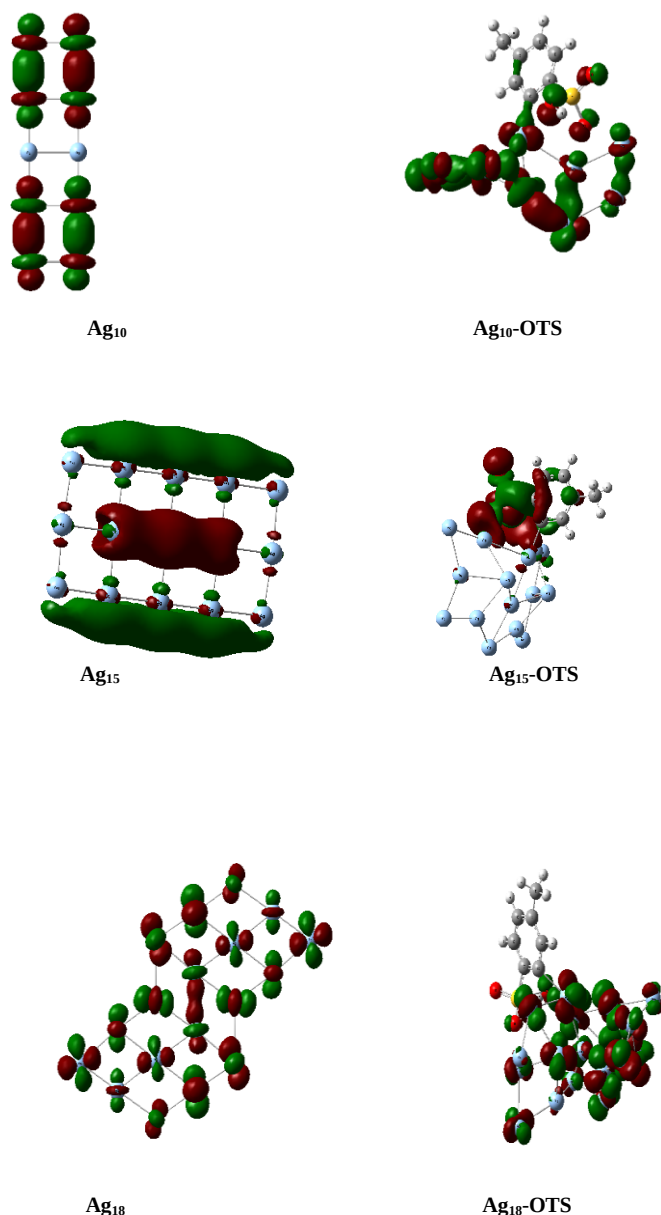
Fig. 2: Electrostatic Potential for ( \text{Ag}_{10} ), ( \text{Ag}_{15} ), ( \text{Ag}_{18} ), ( \text{Ag}_{10}\text{-OTS} ), ( \text{Ag}_{15}\text{-OTS} ) and ( \text{Ag}_{18}\text{-OTS} ).
