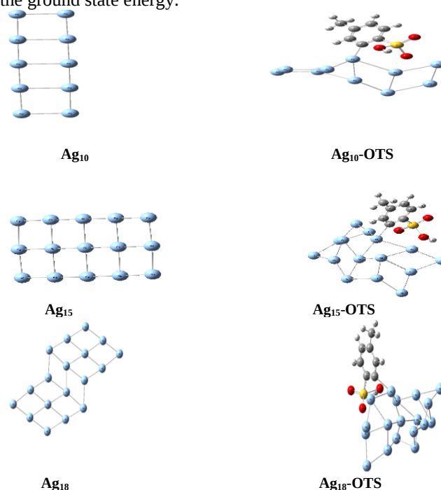
Fig. 1: Molecular structure for ( \text{Ag}_{10} ), ( \text{Ag}_{15} ), ( \text{Ag}_{18} ), ( \text{Ag}_{10}\text{-OTS} ), ( \text{Ag}_{15}\text{-OTS} ) and ( \text{Ag}_{18}\text{-OTS} ).
