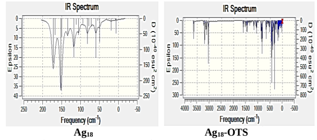
Fig. 4: Infrared spectra schematics for ( \text{Ag}_{10} ), ( \text{Ag}_{15} ), ( \text{Ag}_{18} ), ( \text{Ag}_{10}\text{-OTS} ), ( \text{Ag}_{15}\text{-OTS} ) and ( \text{Ag}_{18}\text{-OTS} ).
