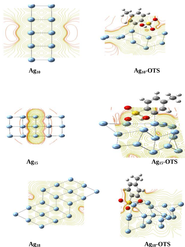
Fig. 3: Charge density distribution for ( \text{Ag}_{10} ), ( \text{Ag}_{15} ), ( \text{Ag}_{18} ), ( \text{Ag}_{10}\text{-OTS} ), ( \text{Ag}_{15}\text{-OTS} ) and ( \text{Ag}_{18}\text{-OTS} ).
