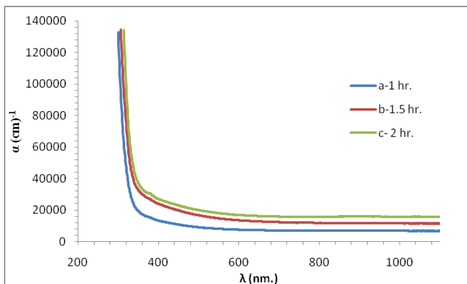
Figure 4: Absorption coefficient of nanocrystalline ZnS thin films versus wavelength at different deposition times: (a) ( t=1 ), (b) ( t=1.5 ) and (c) ( t=2 hr.).
