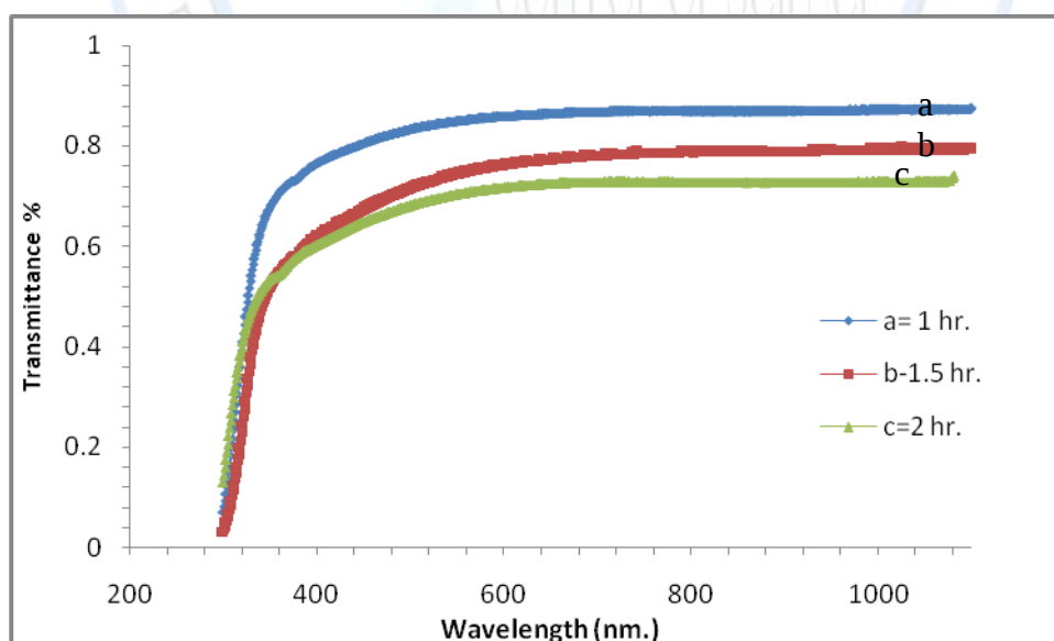
Figure 3: Transmittance spectra of nanocrystalline ZnS thin films versus wavelength deposited at different time: (a) ( t =1), (b)( t =1.5) and (c)( t=2 hr.).
