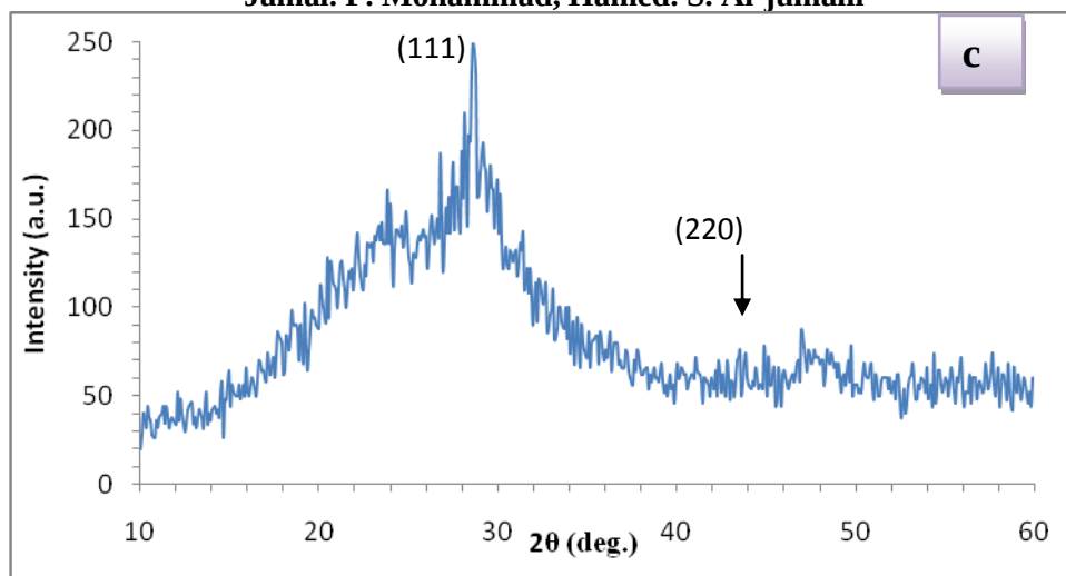
Fig. 2: The X-ray diffraction pattern of as-deposited ZnS on glass substrate at (80 °C) temperature for different deposition time: (a)( t=1), (b) (t=1.5) and (c) t=2 hour.
