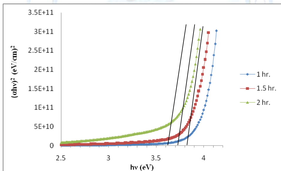
Figure 5: Optical band gap of nanocrystalline ZnS thin films versus photon energy at different deposition time: (a) ( t=1 ), (b) ( t=1.5 ) and (c) ( t=2 hr.).
