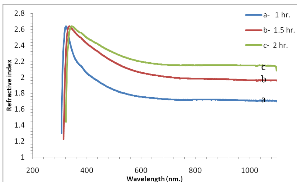
Figure 6: Refractive index of nanocrystalline ZnS thin films versus wavelength at different deposition times:(a) (t =1), (b) (t =1.5) and (c) (t=2 hr.).
