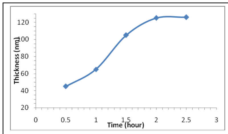
Figure 1: shows variation of ZnS film thickness with different deposition time
