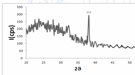
Figure (1): XRD glass
