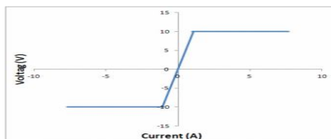
Figuer(6):The I-V characterization of nano Ag thin film( 60,65)nm on glass substrat.
