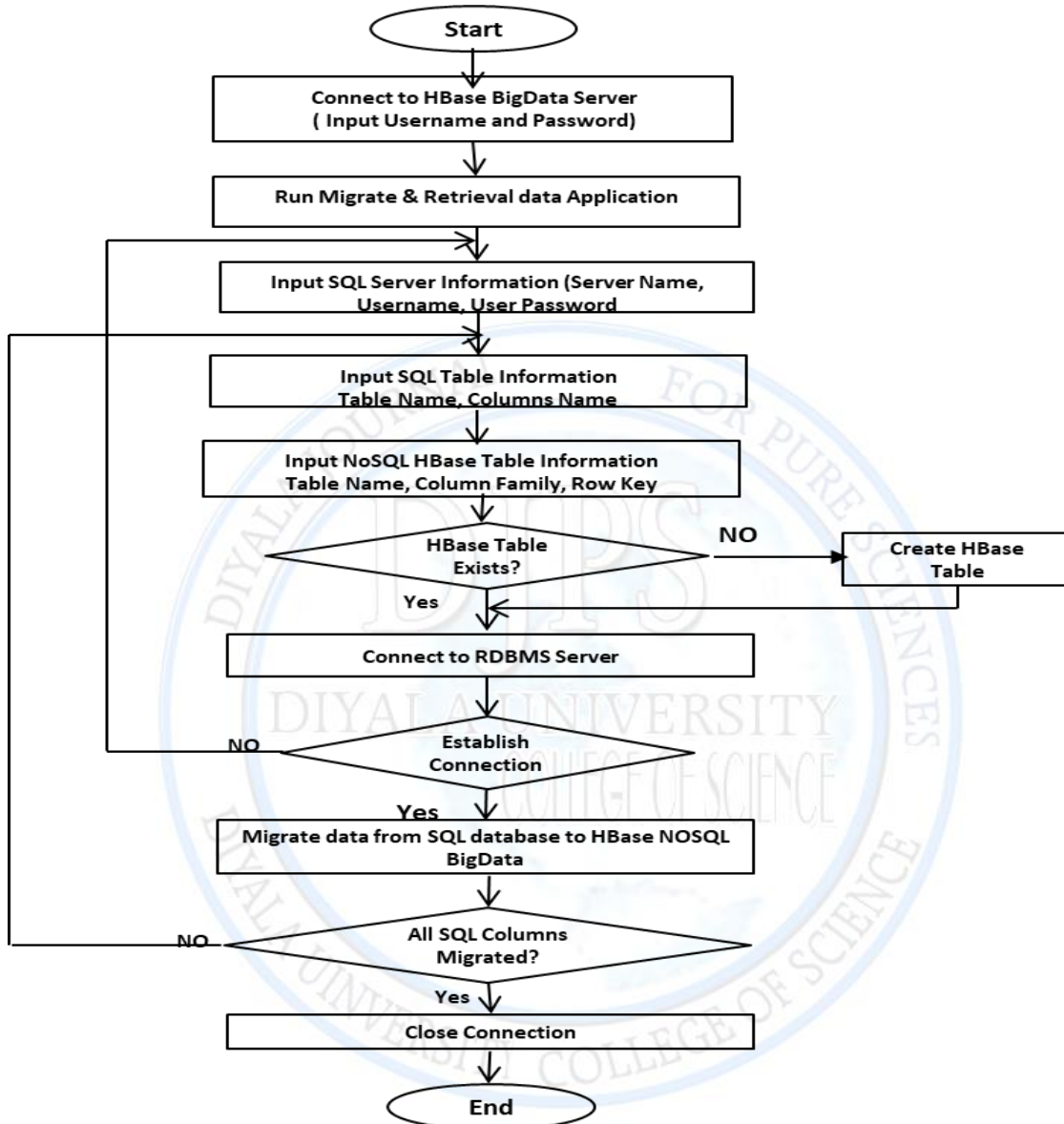
Figure 4: Flowchart of data conversion and migration process.
