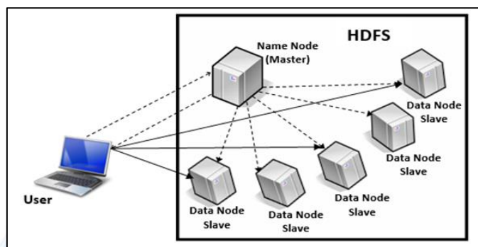
Figure 1: HDFS Architecture [18]
