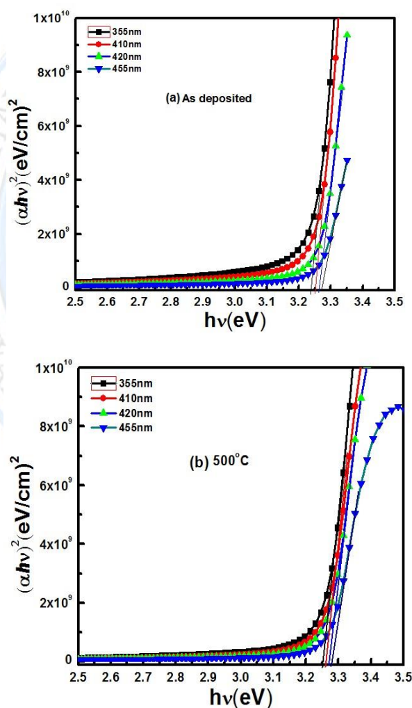
Figure 5: The typical variation of (\alpha h\nu)^2 versus photon energy of ZnO thin films, (a) without and (b) with annealing.
