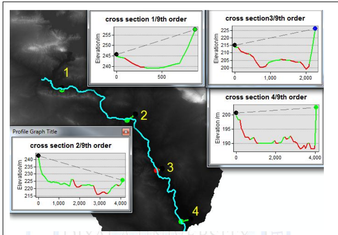
Figure (4A): valley shape for order 9.
