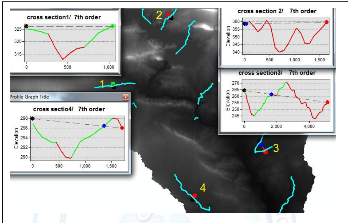
Figure (4C): valley shape for order 7.
