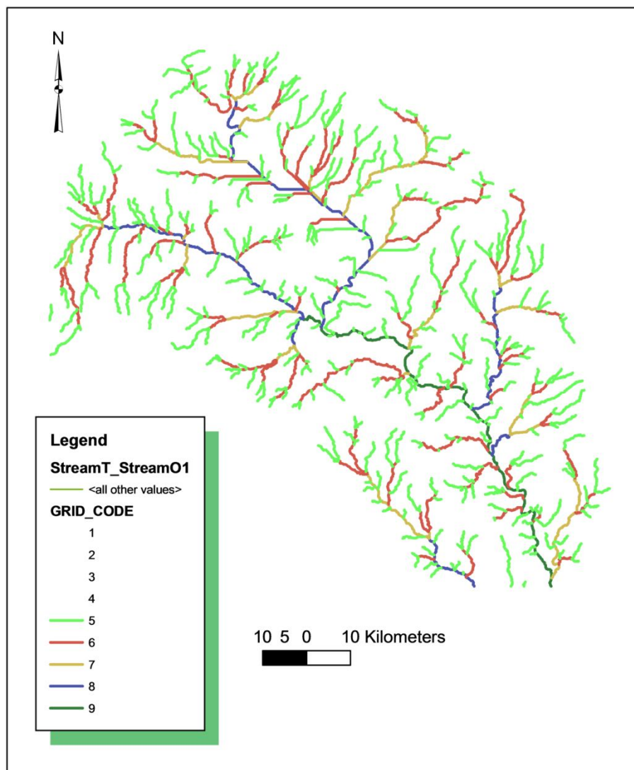
Figure 3: stream orders of the study area.
