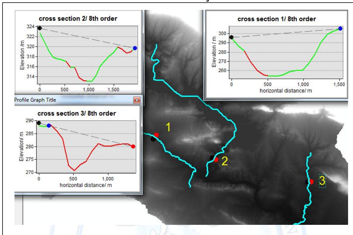
Figure (4B): valley shape for order 8.
