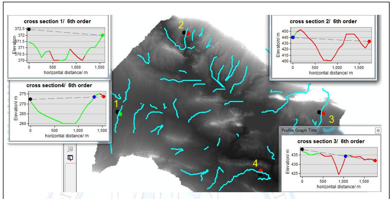
Figure (4D): valley shape for order 6.
