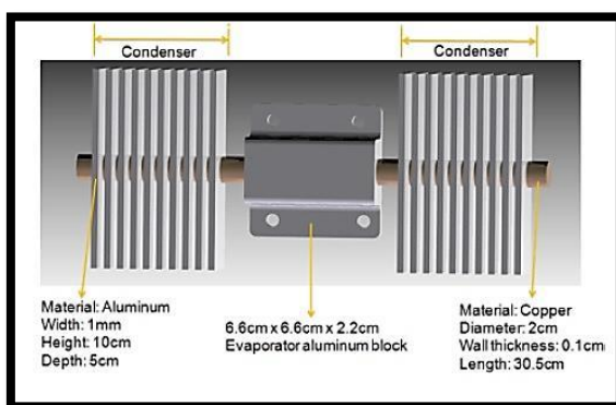
Figure 2. Fin arrangement on heat pipe.
