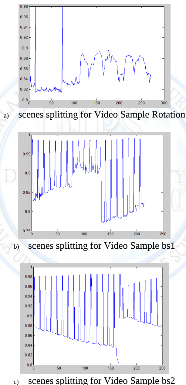
Figure 4: Scenes splitting
