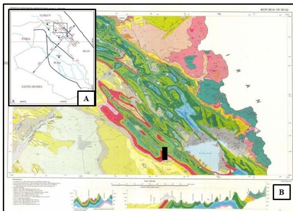
Fig. 1: Location Maps: (A) Tectonic map of Iraq showing the tectonic subdivision zones. (SSZ: Sanandaj-Sirjan Zone; ZFTB: Zagros Fold-Thrust Belt; MZ: Mesopotamian Zone; SSh: Stable Shelf (after [5-6- 7])), B- Geological map of northeast Iraq showing the location of studied section (Haibat Sultan).
