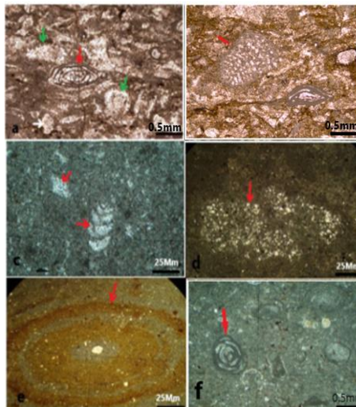
Fig. 6: Photomicrograph a Fossiliferous packstone showing deformed Miliolid due to compaction process, b- Dictyoconus aidymi in fossiliferous packstone (red arrow). c- Fossiliferous Mudstone to wackestone showing small benthic foram, Textularia sp. is affected by the micritization processing, and Rotalia sp. is affected by neomorphism. d – Burrowed Mudstone to wackestone showing the burrows filled by skeletal and non-skeletal grains. E- Oncoidal wackestone to packstone. f- Fossiliferous wackestone showing Miliolid (red arrow).
