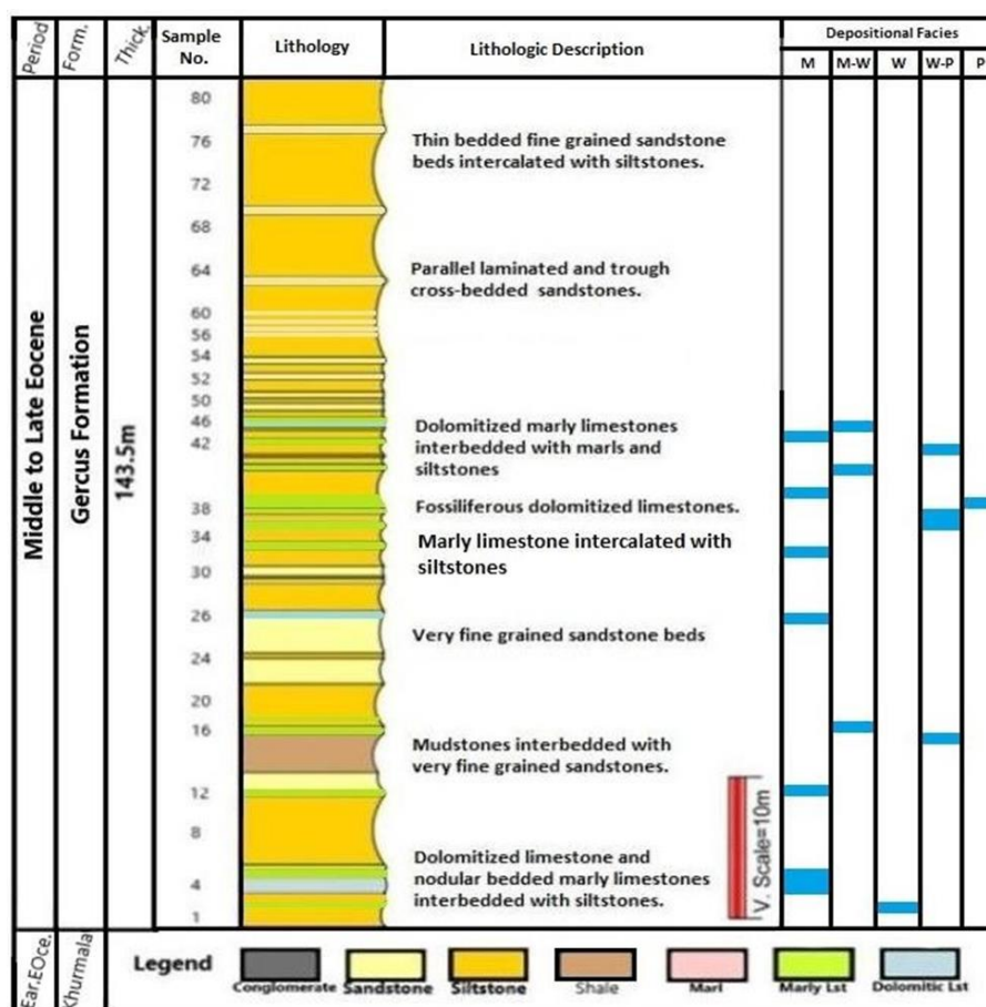
Fig. 3: Geologic column showing lithologic descriptions and depositional facies of the Avanah carbonate rock interbeds within the lower and middle parts of the Gercus Formation at Haibat Sultan section.
