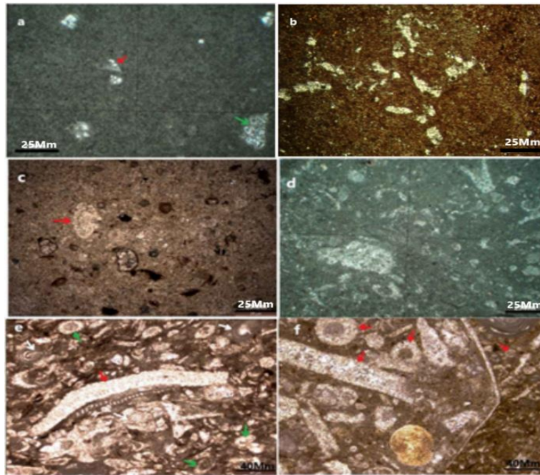
Fig. 5: Photomicrograph a- Fossiliferous mudstone, b- Argillaceous Mudstone with grains of dolomite. c- Peloidal fossiliferous wackestone to packstone (Rotaliid). d – Bioclastic fossiliferous wackestone to packstone. e- Fossiliferous packstone showing Orbitolites sp. (red arrow). f- Fossiliferous packstone showing dasycladacean green algae (red arrows).
