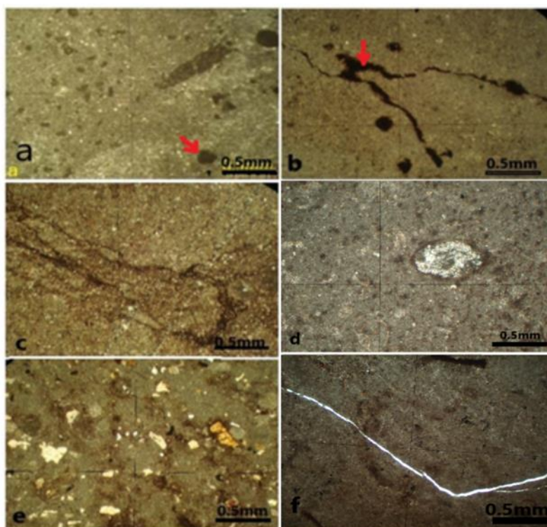
Fig. 4: Photomicrograph showing a-Peloids in Peloidal wackestone (Red arrow), b-Bituminous Mudstone. c- Brecciated mudstone. d- Ostracode in micritic matrix. e- Extraclasts Mudstone. f-Laminated Mudstone to wackestone.
