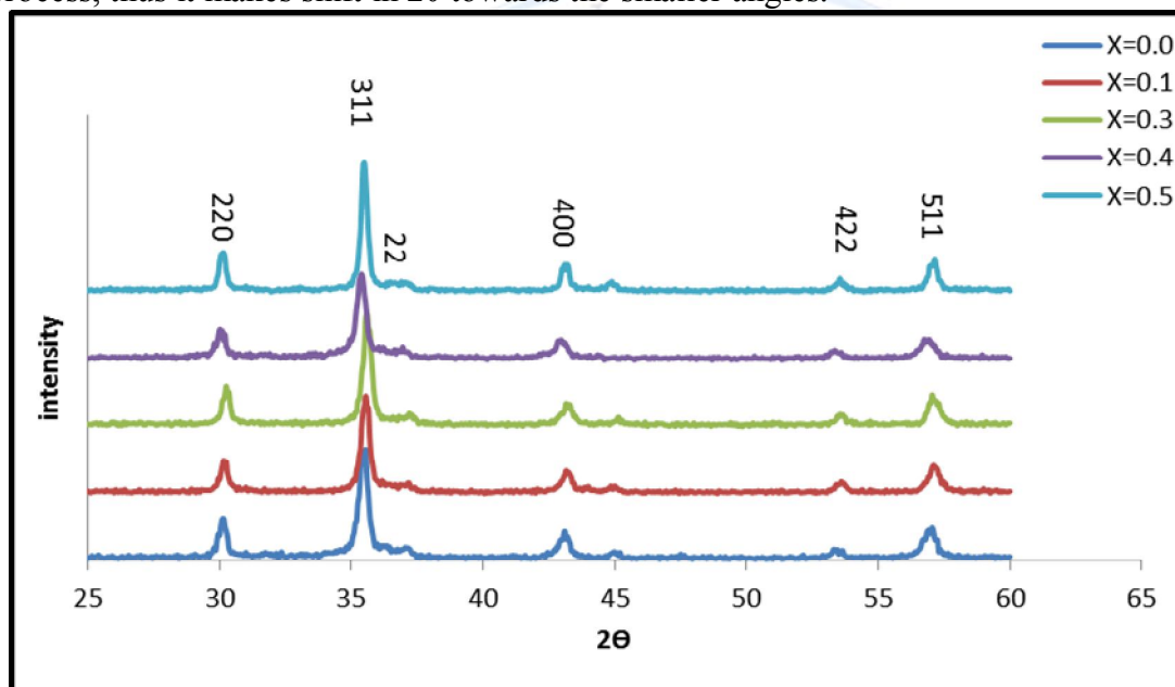
Fig. (1) XRD pattern of the x=0.0, 0.1, 0.3, 0.4, 0.5 at 200^\circ\text{C} for ferrite powder).
