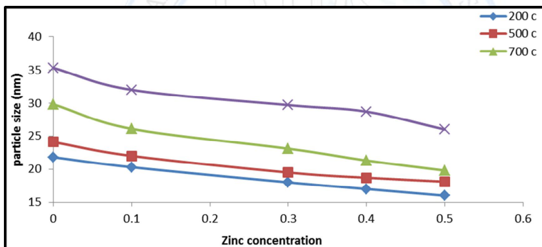
Fig (2) change in the particle size with the degree of zinc substitution in \text{Co}_{1-x}\text{Zn}_x\text{Fe}_2\text{O}_4 ( X=0.0-0.5 ).
