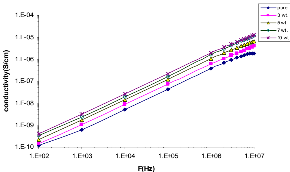
Figure.5. Variation of A.C electrical conductivity for (PVA- BaSO 4 .5H 2 O) composite with Frequency
