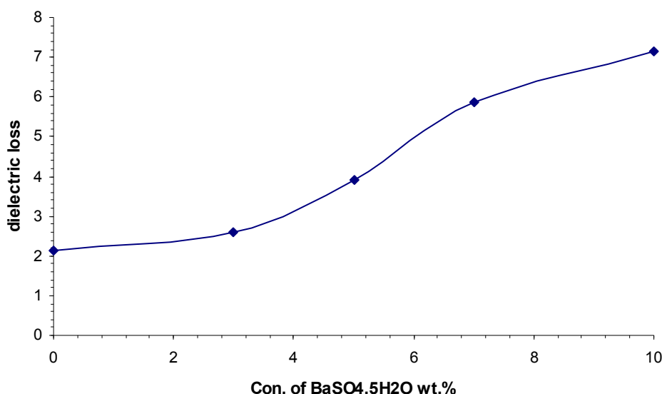
Figure.5. Effect of \text{BaSO}_4 \cdot 5\text{H}_2\text{O} concentration on dielectric loss for composite at 100Hz.
