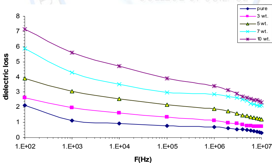
Figure.3. Variation of dielectric loss for (PVA- \text{BaSO}_4 \cdot 5\text{H}_2\text{O} ) composite with Frequency
