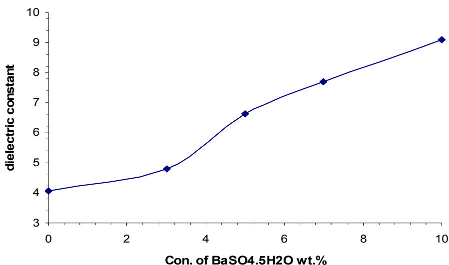
Figure.2. Effect of \text{BaSO}_4 \cdot 5\text{H}_2\text{O} concentration on dielectric constant for composite at 100Hz.
