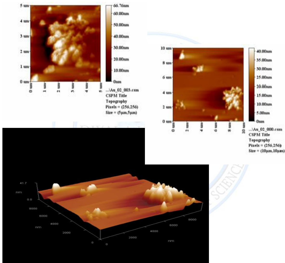
Fig.(11,12) : AFM images with 3D image of Au nano-powder ,prepared by electrochemical method.
