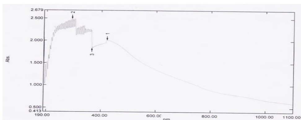
Fig.(7): UV-visible spectroscopy of gold nano particals solution synthesis.
