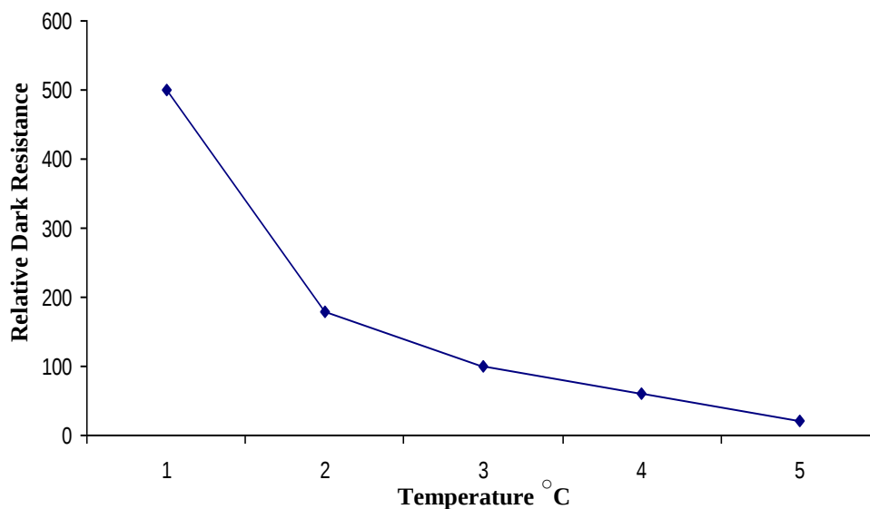
(Fig 11): Relation between relative dark resistance and Temperature °C
