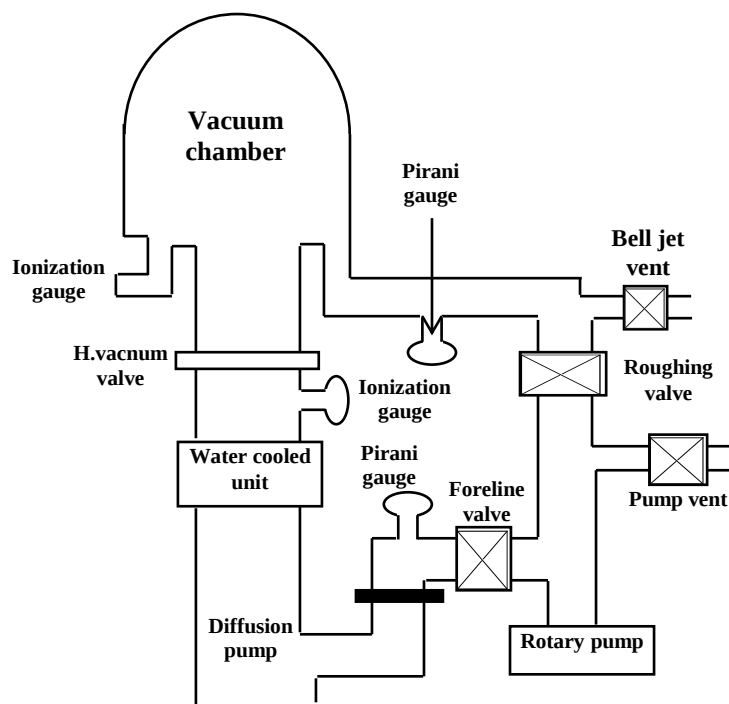
Figure (1) the typical coating system
