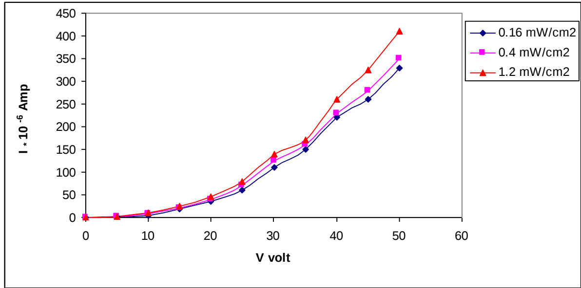
Figure (8) the current-voltage in lumen's stat.
