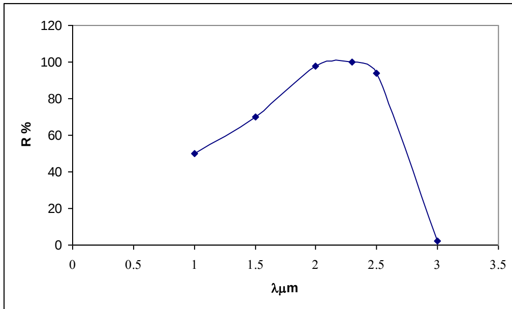
Figure (9 ) shows the spectral responsivity as function of wavelength.
