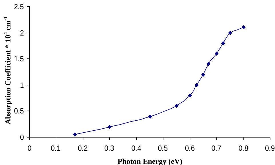
(Fig 5): Relation between Absorption Coefficient and Photon Energy Figure ( 6 ) showed the absorption coefficient increasing with decreased in incident photon energy. This coefficient increases when the photon energy greater than (0.42 eV). Also we can observe that from figure the absorption coefficient decreases with the increasing of wavelength. The explanation of the shift in the absorption edge to shorter wavelength is attributed to the disappearance of the subsidiary band which suggests from the dispersion theory that confirms the bredding of the absorption edge by growth in grain size that causes a decrease in the thermal excitation of electrons lying in the levels associated with this band at room temperature and an increase in the energy gap between valance band and conductor band leading to decrease in the absorption coefficient and shift to longer photon energy.
