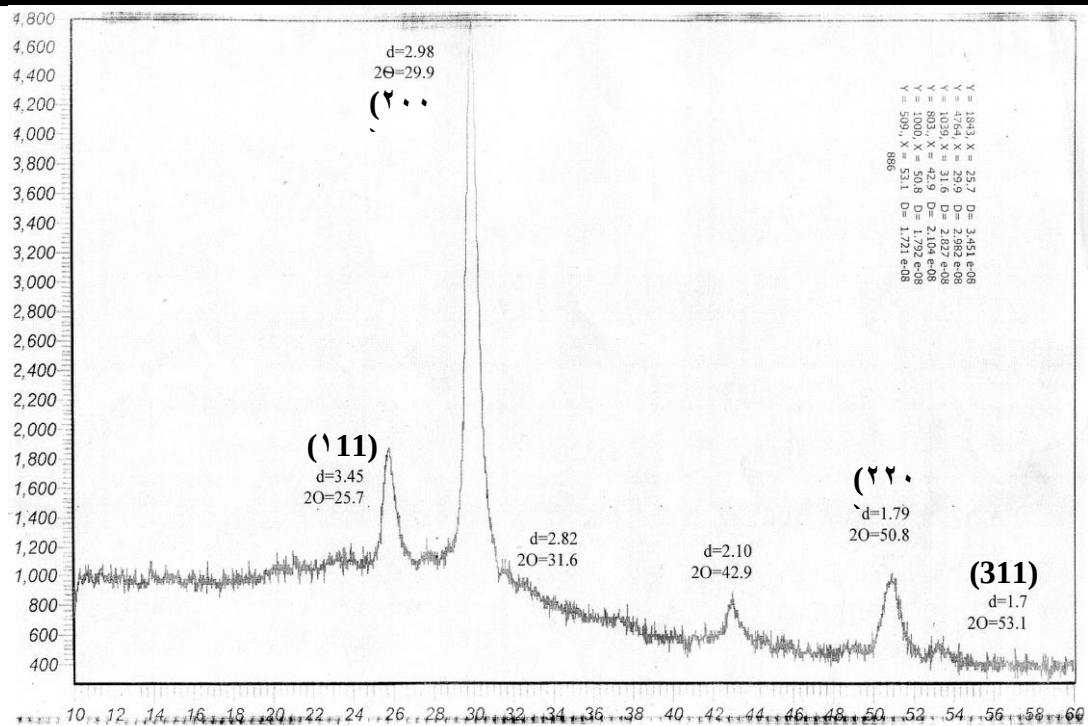
Figure (4) shows the patterns of x-ray diffraction for (PbS) films at room temperature
