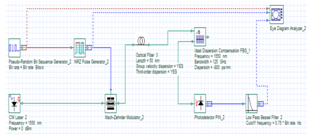
Figure 10. Post-compensation system.
