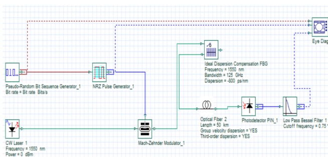
Figure 9. Pre-compensation system.
