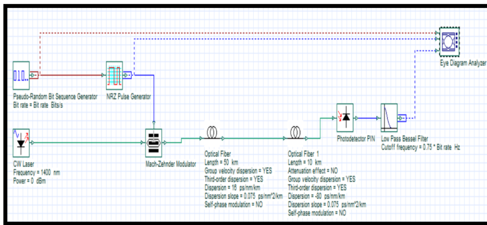
Figure 4. Block diagram of dispersion compensation fiber in Opti System
