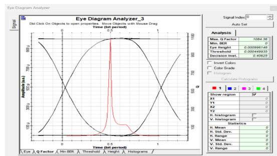
Figure 14. Symmetric compensation signal eye diagram
