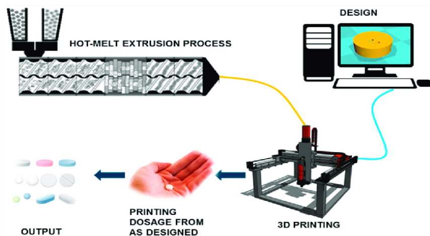
Figure 4: Hot Melt Extrusion process
