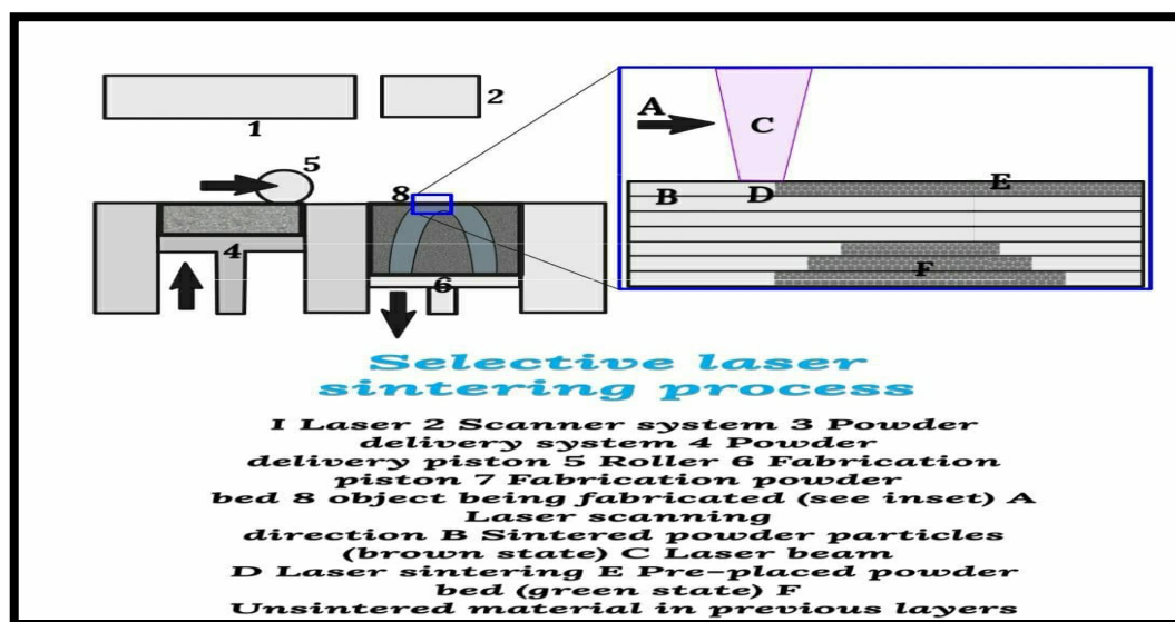
Figure 2: Selective laser sintering process
