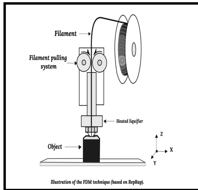
Figure 3: Illustration of the FDM technique
