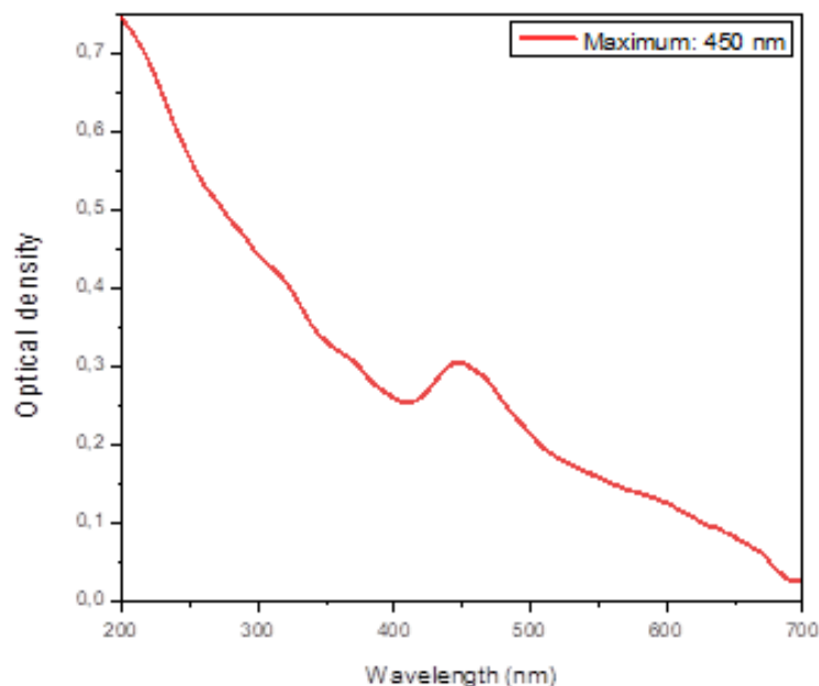
Figure 5: UV-visible absorption spectrum of silver nanoparticles (appearance of a surface plasmon resonance band between 400 and 500 nm).
