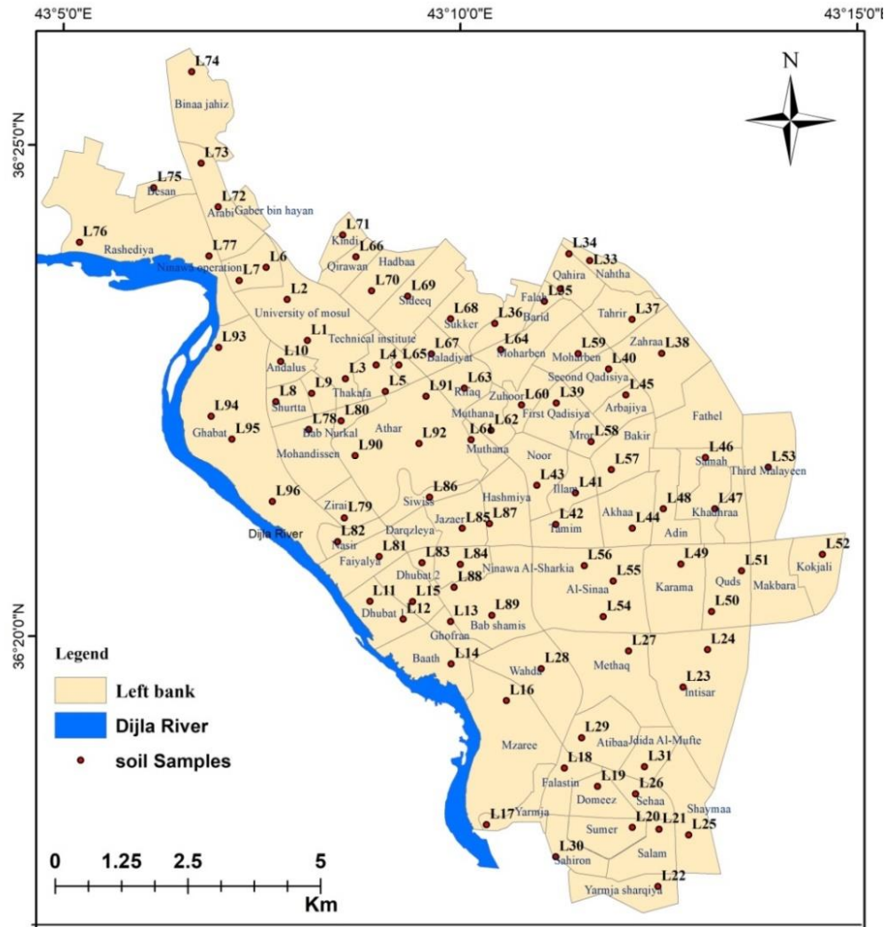
Fig. 2. Location map of soil samples in the studied area.
