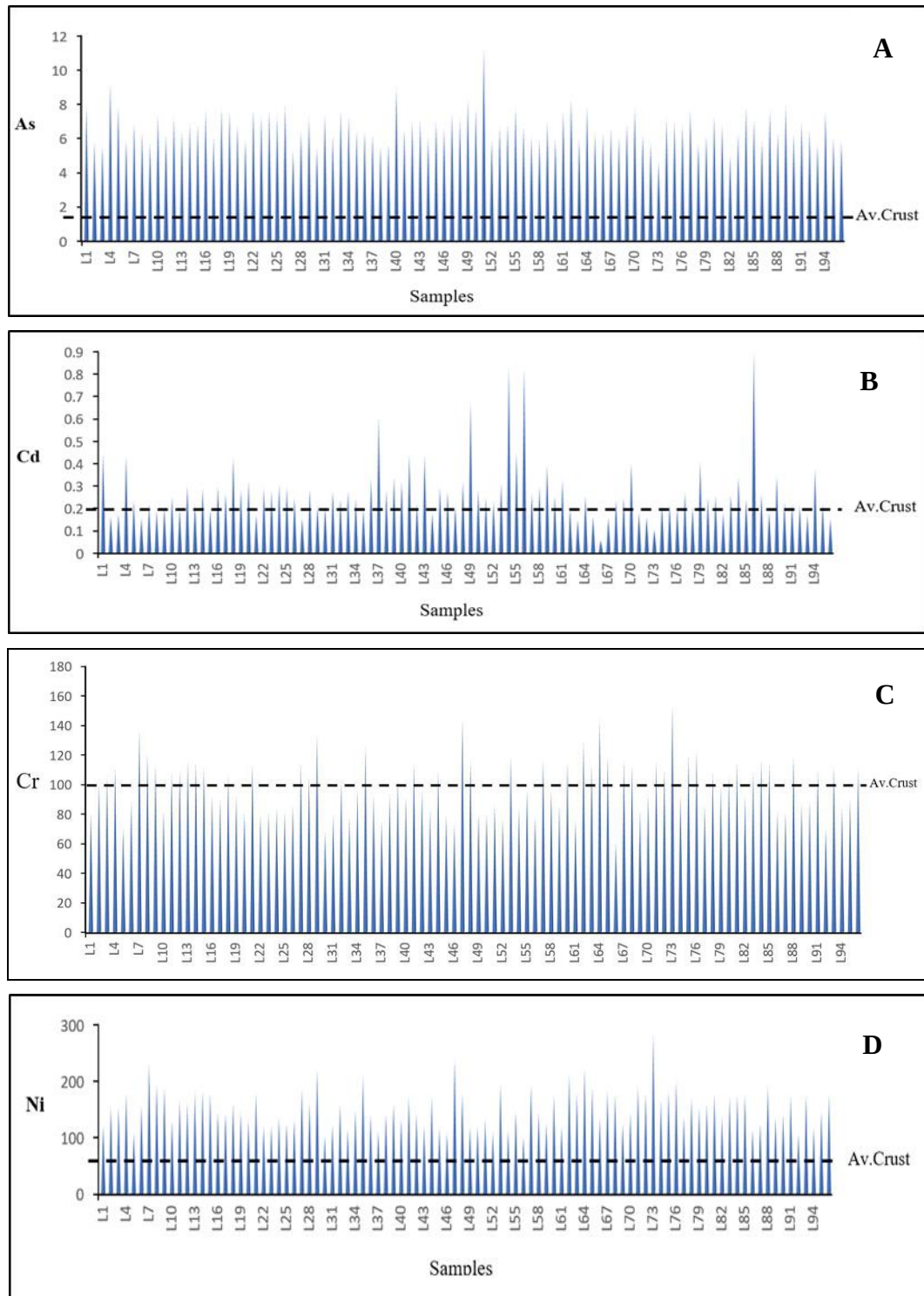
Fig. 4. Heavy metals in the soil samples from the left bank.
