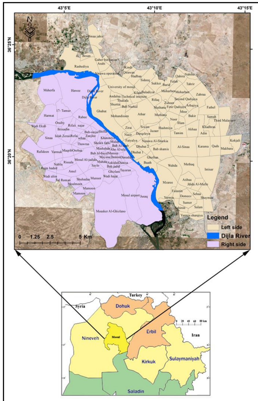
Fig. 1. Location map of Mosul City (modified from Mosul-Municipalities, 2022)
