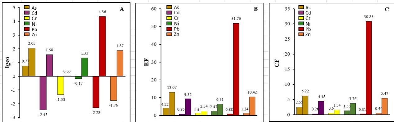
Fig. 5. Minimum and maximum values of (A) geo-accumulation index ( I_{geo} ), (B) enrichment factor (EF), and (C) contamination factor (CF) of soil heavy metals in the left bank study area
