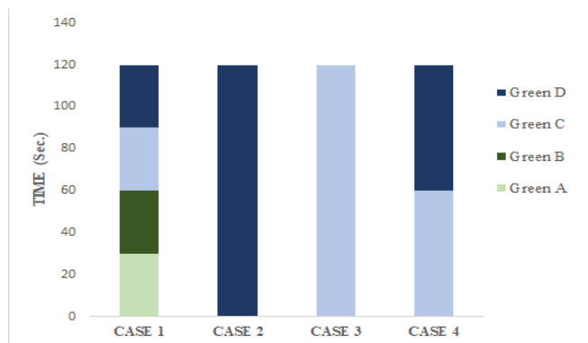
Fig. 7. Group 1 Green signal time
