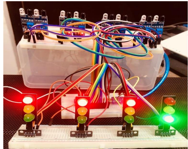
Fig. 4. Prototype Circuit
