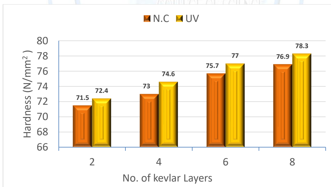
Figure 6: The comparison of hardness with the number of Kevlar fiber layers in the mixture before and after UV irradiation
