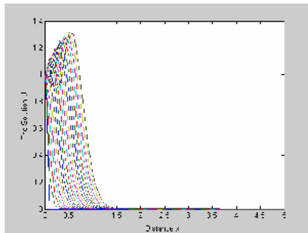
Fig.(2): Numerical approximation of the Crank-Nicolson F.D.M. for the first problem
