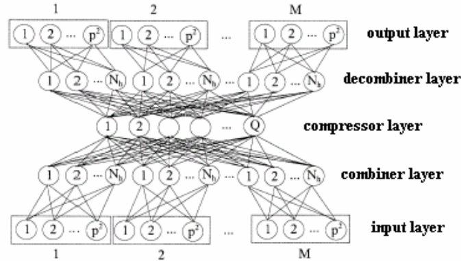
Fig. (1) Hierarchical neural network structure.
