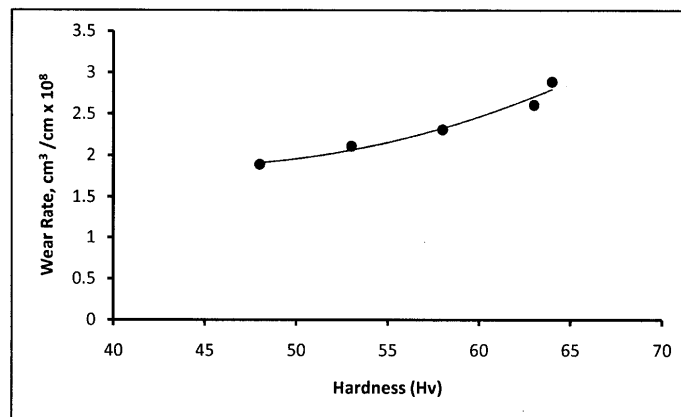
Fig. 5 The relationship between hardness and wear rate of Al-Si-Pb alloys. Sliding distance, 40.37 km.
