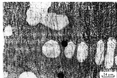
Al-12%Si-1%Pb
