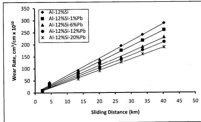
Fig. 3 The relationship between sliding distance and wear rate of Al-Si-Pb alloys.
