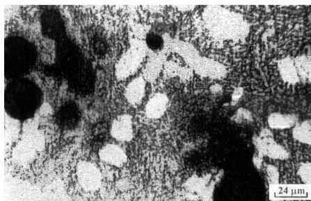
Al-12%Si-20%Pb
