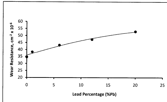
Fig. 4 The relationship between lead percentage and wear resistance of Al-12%Si alloy. Sliding distance, 40.37 km.
