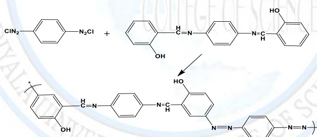
Scheme 6: The preparation of polymers
