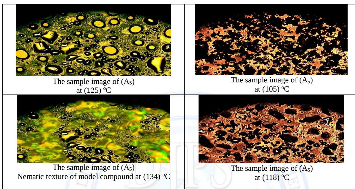
Figure 7: The sample images of (A 5 ) in hot stag polarized light microscopy at different temprature
