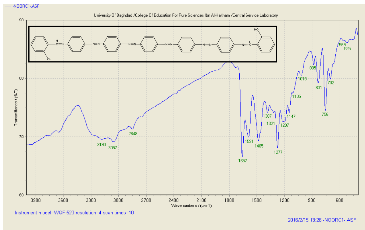
Figure 4: FTIR spectrum of (C 1 ) compound
