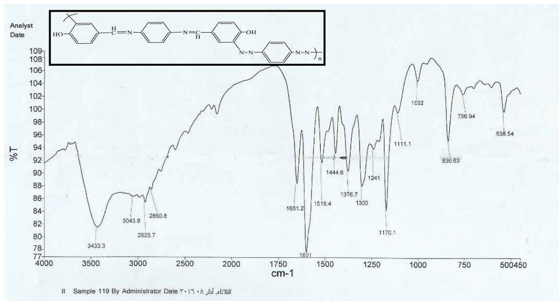
Figure 5: FTIR spectrum of (II) Polymer
