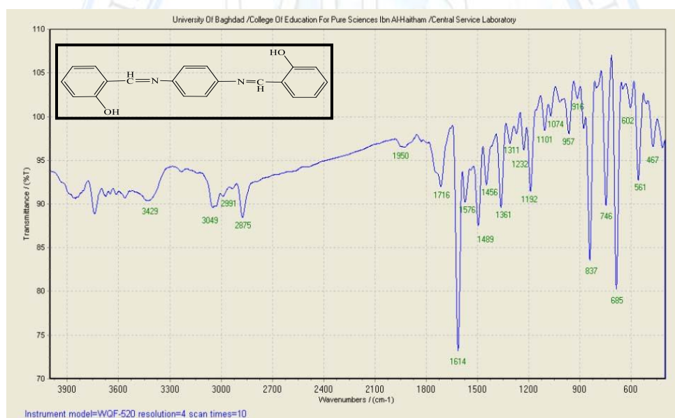
Figure 1: FTIR spectrum of (A 1 ) compound
