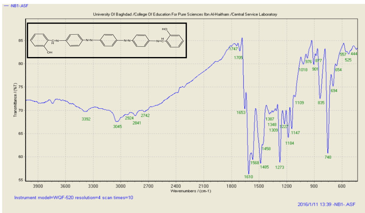
Figure 3: FTIR spectrum of (B 1 ) compound
