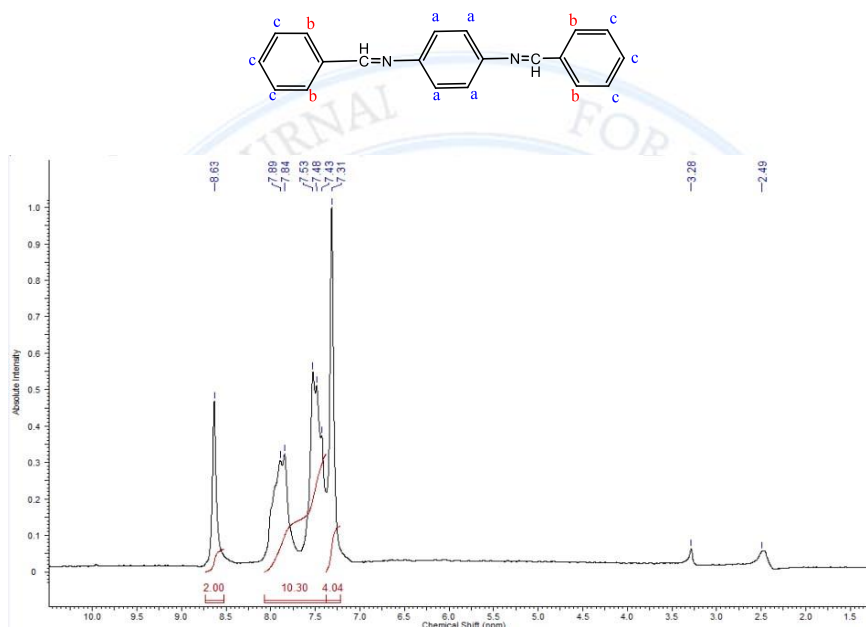
Figure 2: ^1\text{H} -NMR spectrum of ( \text{A}_5 ) compound
