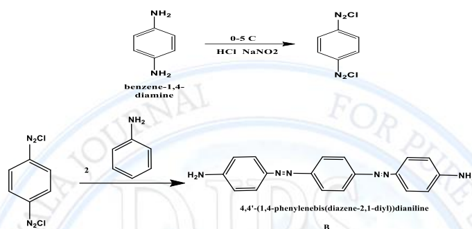
Scheme 1: The preparation (B) compound
