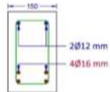
Sec. E-E
