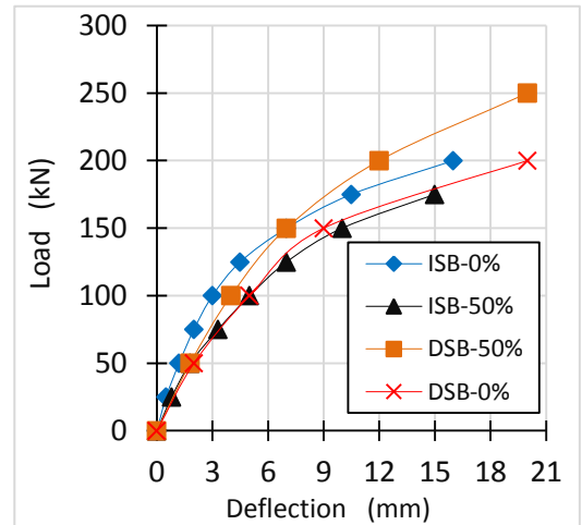
Figure 7: Comparison of Load Versus Mid-Span Deflection Curve for DSB and ISB Beams
