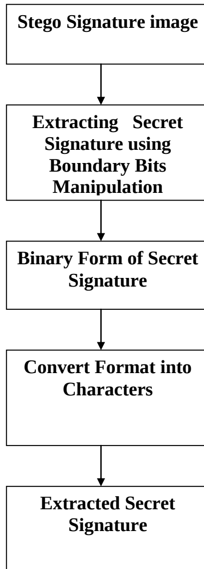
Figure (3) Block Diagram of Extracting Side for Simple Binary Image Steganography Model
