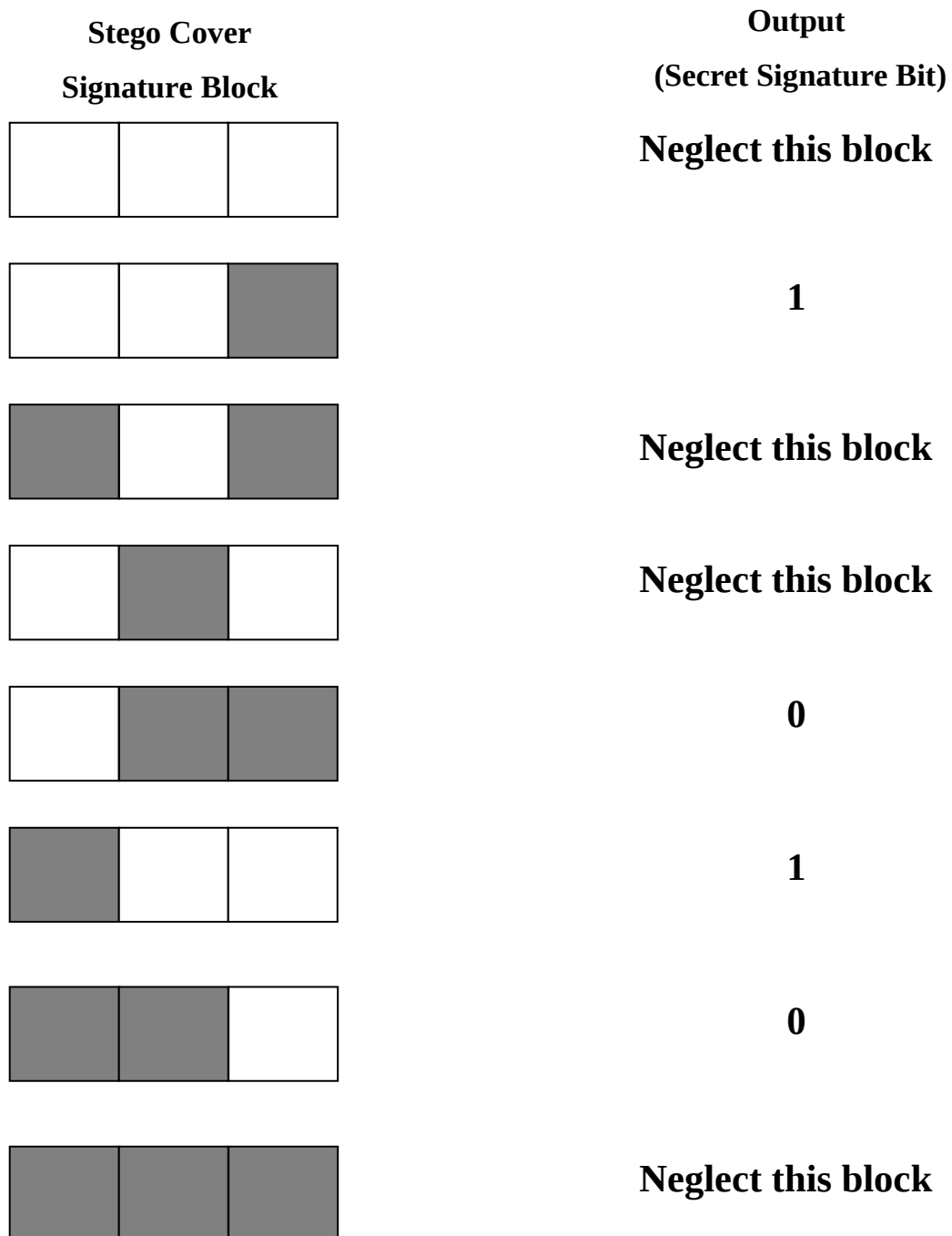
Figure (4) The Idea of Extracting Technique Using 3-Bit Manipulation. Black Represents 0 and White Represents 1.
