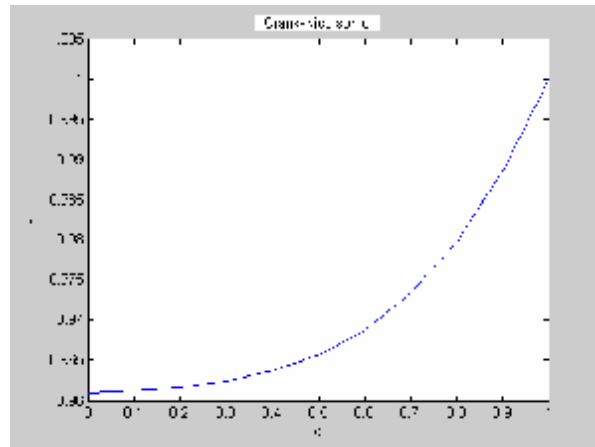
Figure (3) an illustration of the solution of (2.1) by Crank-Nicolson Method. The solution for u_{11} is plotted as a function space x at successive time t , with the parameters v_0=0.1 , g=0.05 , b=30 .
