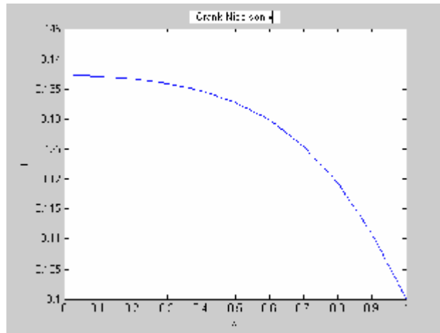
Figure (4) an illustration of the solution of (2.1) by Crank-Nicolson Method. The solution for v_{11} is plotted as a function space x at successive time t , with the parameters v_0=0.1 , g=0.05 , b=30 .
