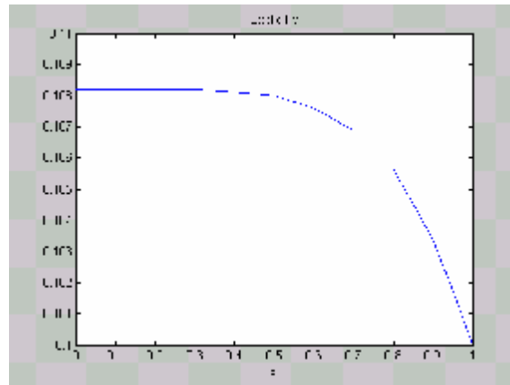
Figure (2) an illustration of the solution of (2.1) by Explicit method. The solution for v_{11} is plotted as a function space x at successive time t , with the parameters v_0=0.1 , g=0.05 , b=30 .
