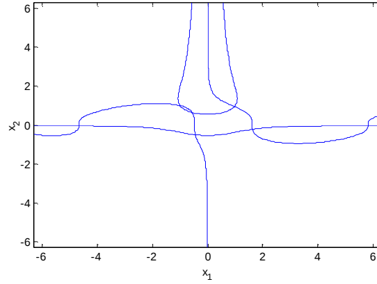
Fig (2). System of the two equations above.
