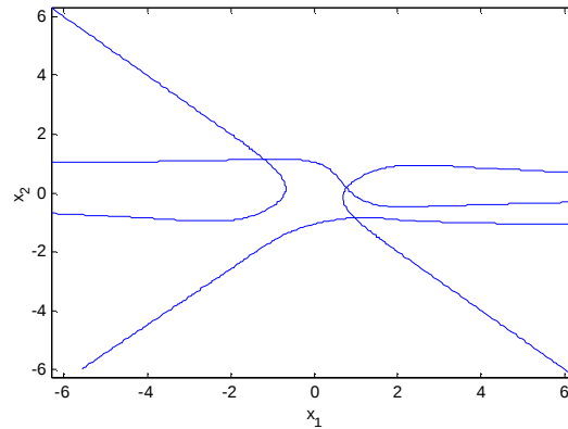
Fig (1): System of the two equations above.
