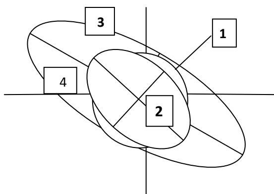
Fig (4) polarization characteristics of the He-Cd 4416 Å laser line in WAMF, 1: H=0 Gauss , 2: H=2 Gauss, 3: H=5 Gauss, 4: H=6 Gauss.
