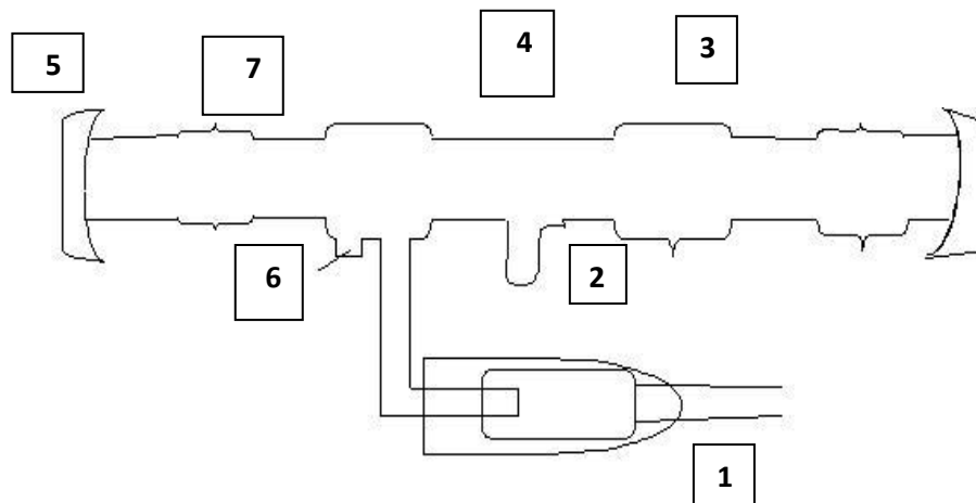
Fig(2) structure of laser tube,1-cathode,2-cd oven,3-anode,4-active bore 5-mirror,6-auxiliary anode,7-bellows.
