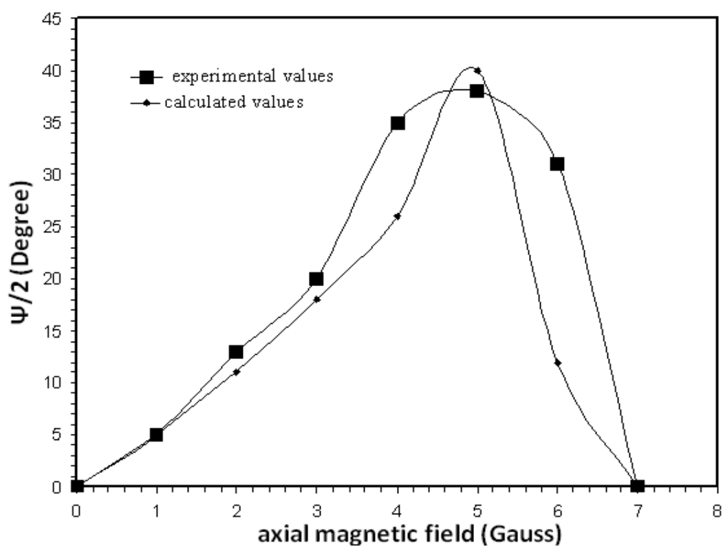
Fig(3) angle of the polarization axis \Psi/2 versus strength of WAMF.
