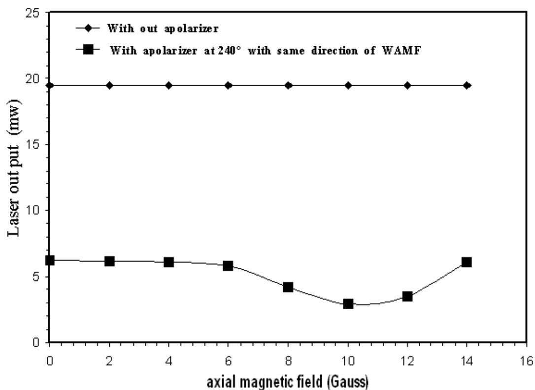
Fig.(6b).laser output as a function of the WAMF strength,(■) with a polarizer at 240° with same direction of WAMF, (◆) with out polarized . Table(2) laser output as a function of the WAMF strength with a polarizer at 150° , 240°with same direction of WAMF ,and 240° with reversed direction of WAMF,and also without polarizer.
