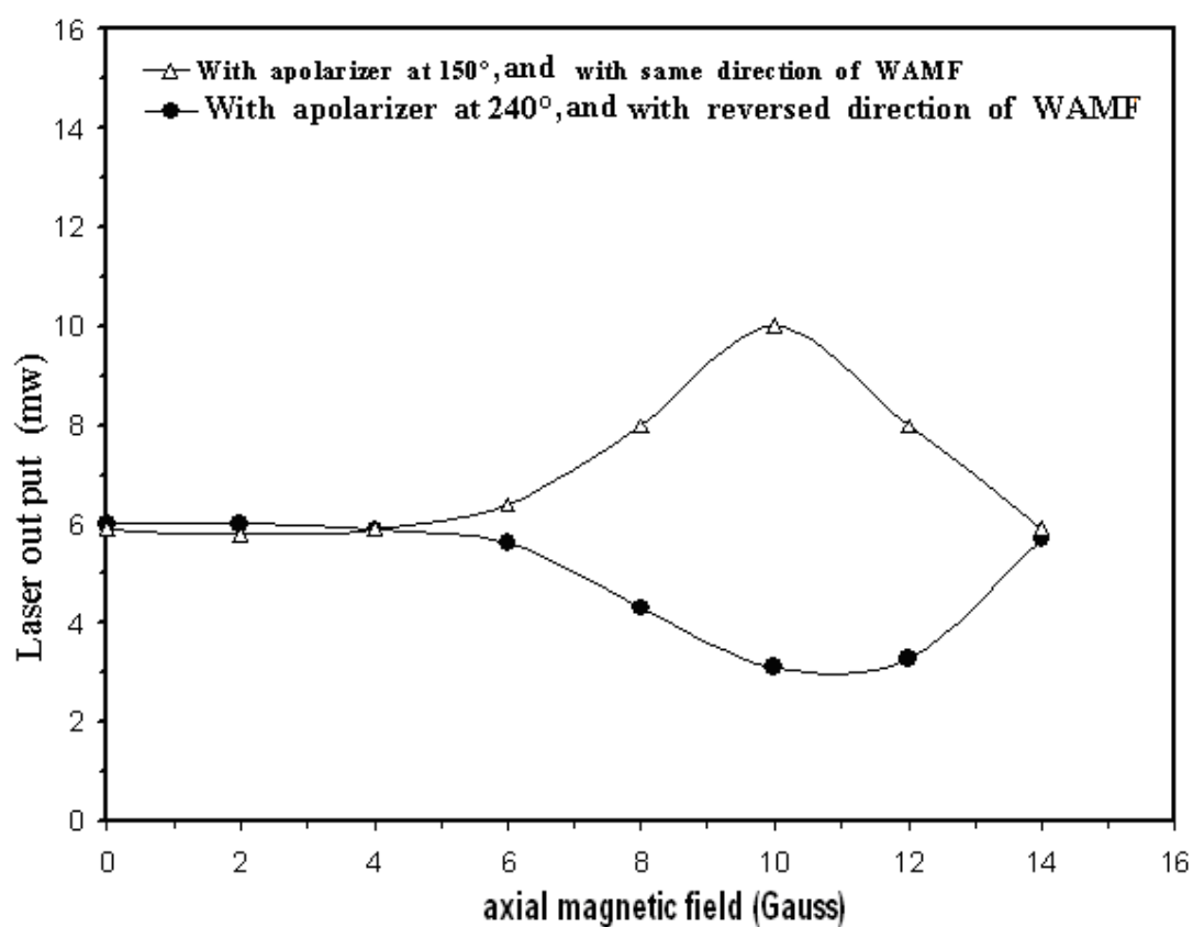
Fig.(6a).laser output as a function of the WAMF strength, ( \Delta ) with a polarizer at 150^\circ with same direction of WAMF, and ( \bullet ) with a polarizer at 240^\circ with reversed direction of WAMF.
