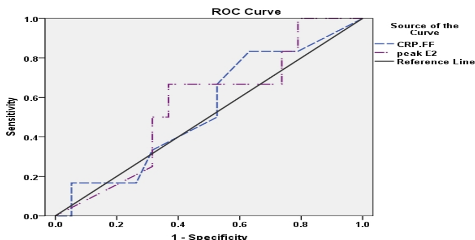
Figure 4: Estimated area under curve (AUC) and predictive cut-off point values for the individual some seroimmunological and hormonal parameters with the receiver operating characteristics (ROC) curve analysis between pregnant and non-pregnant women
