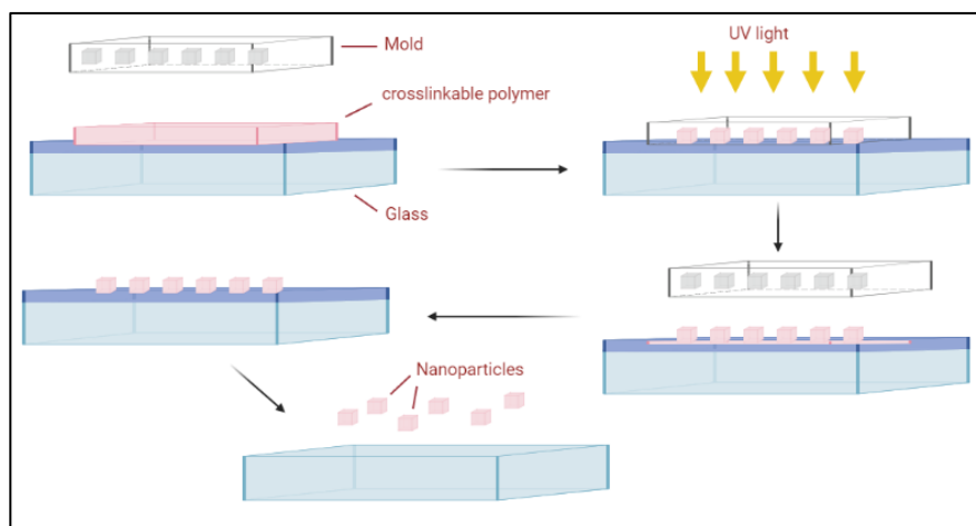
Figure 6: Photolithographic Techniques
