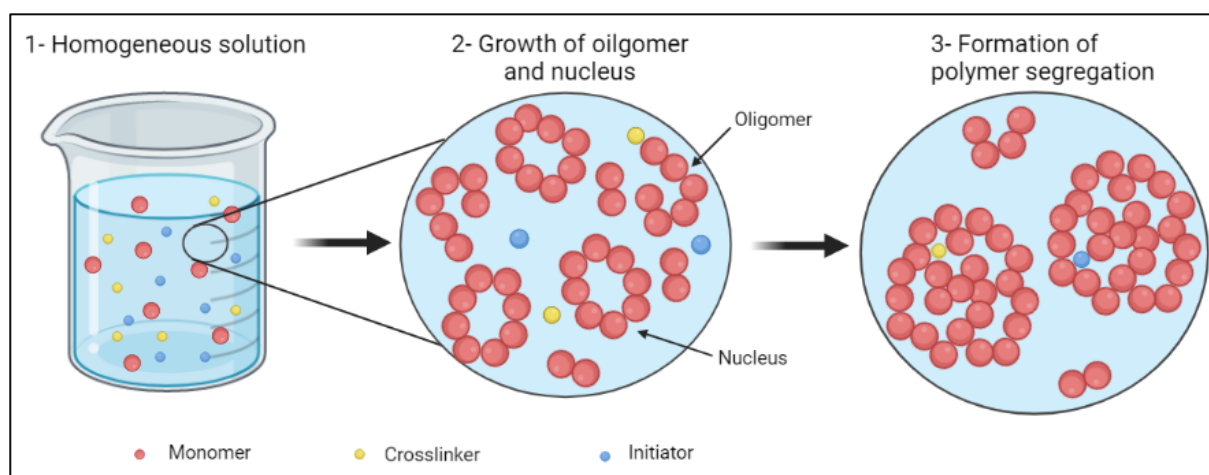
Figure 7: Precipitation polymerization
