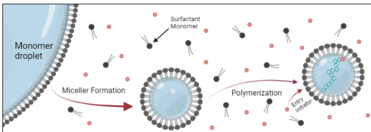
Figure 2: Emulsion Polymerization Technique
