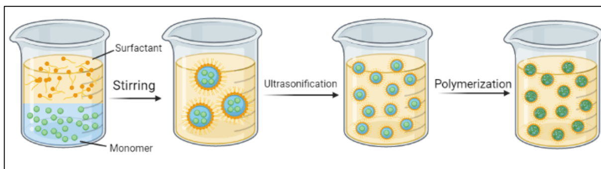
Figure 3: Inverse mini emulsion polymerization
