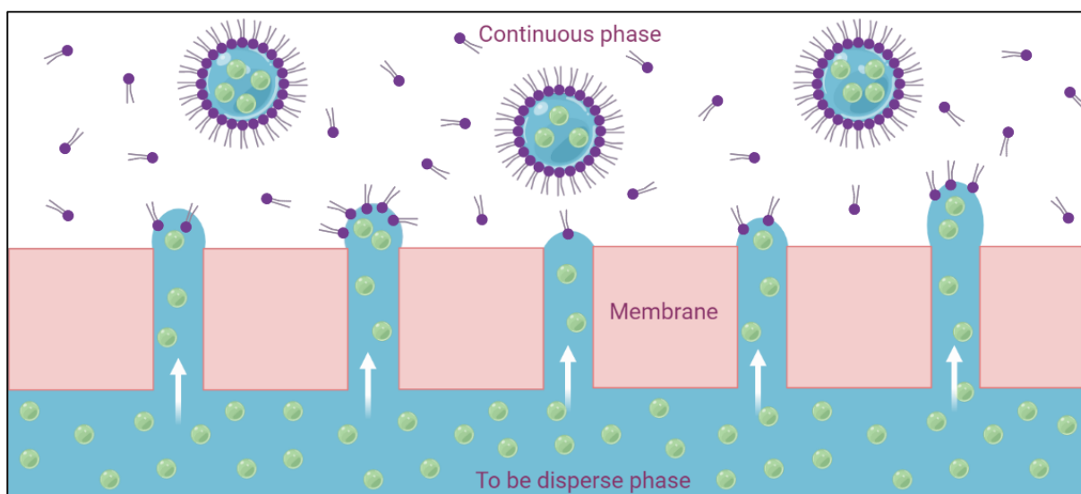
Figure 5: Membrane emulsification
