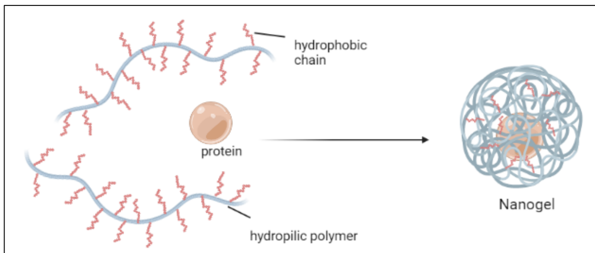
Figure 1: Physical Self-Assembly
