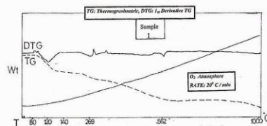
Fig(6) Thermogravimetric analtsis of polymer Ligand p - hydroxybenzoic acid ureaformaldehyde
