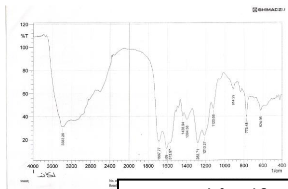
Fig(10 ) Infrared Spectrum of the polymer : Chelate p- hydroxybenzoic acid ureaformaldehyde with Sr II
