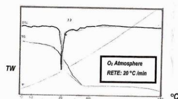
Fig(4) Thermogravimetric analtsis of polymer Chelate p - hydroxybenzoic acid ureaformaldehyde with Ba^{II}
