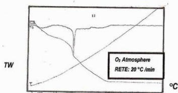
Fig(5) Thermogravimetric analtsis of polymer Chelate p - hydroxybenzoic acid ureaformaldehyde with Sr^{II}
