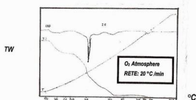
Fig(3) Thermogravimetric analtsis of polymer Chelate p - hydroxybenzoic acid ureaformaldehyde with Ca^{II}
