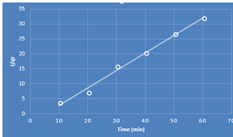
Figure 6: Pseudo-second order reaction for chromium onto nanocomposite TR-TiO 2 -2.
