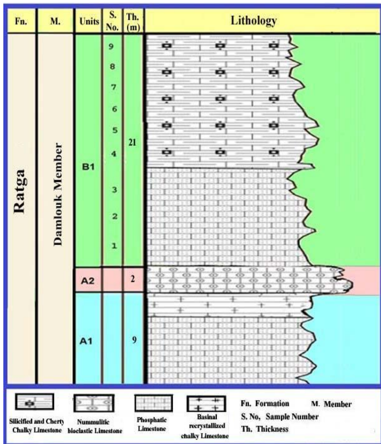
Fig. 3: Lithostratigraphic column of the studied part of the Damlouk Member, Ratga Formation, W. Iraq.
