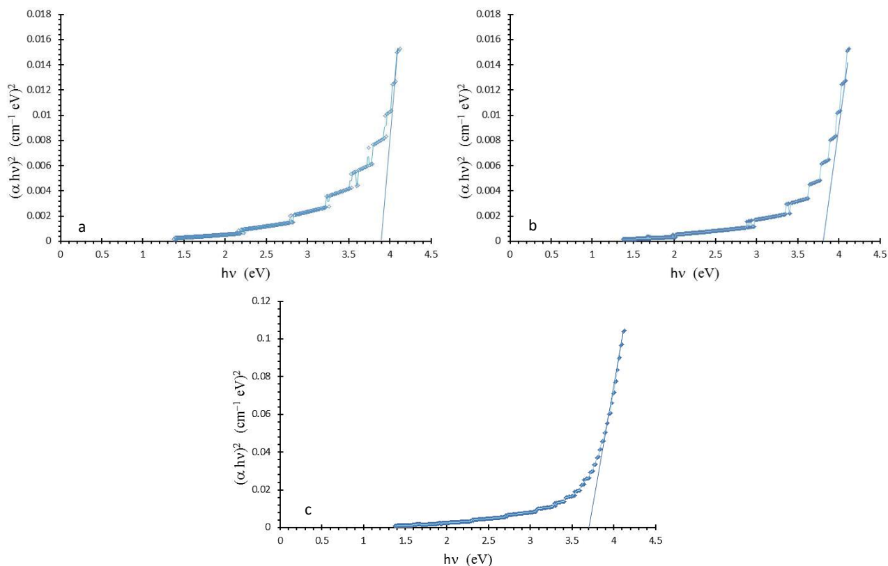
Figure 4: The optical band gap of \text{TiO}_2 NPs prepared at different laser energy (a) 80mJ (b) 120mJ, and (c) 160mJ.
