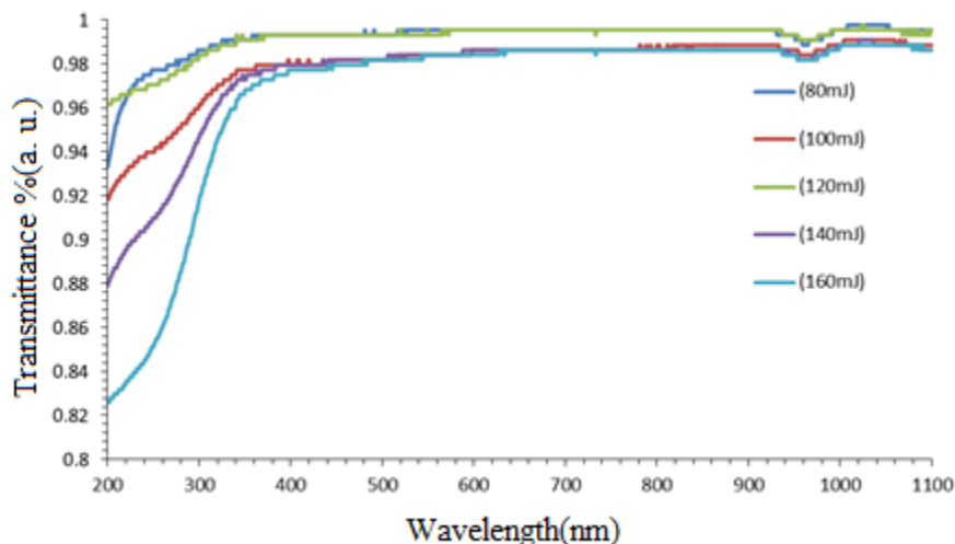
Figure 3: Transmittance spectra of the TiO 2 NPs colloidal synthesised with different laser energy at 100 pulses.
