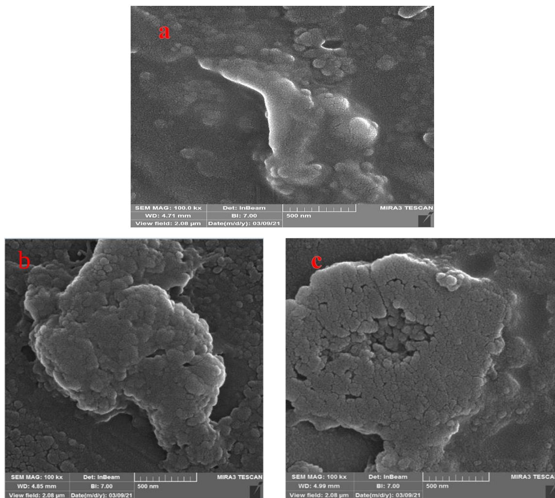
Figure 6: FE-SEM micrographs of \text{TiO}_2\text{NPs} synthesised with laser energy of (a) 80 mJ, (b) 120mJ, and (c) 160mJ at 100 pulses.
