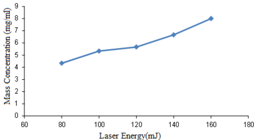
Figure 2: Mass concentration of ablated TiO 2 NPs versus laser energy.
