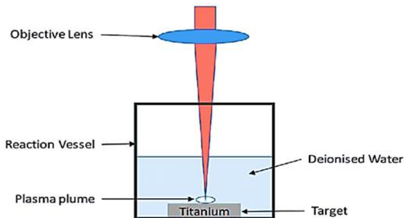
Figure 1: A schematic representation of ablation process of titanium target in water by laser [10].
