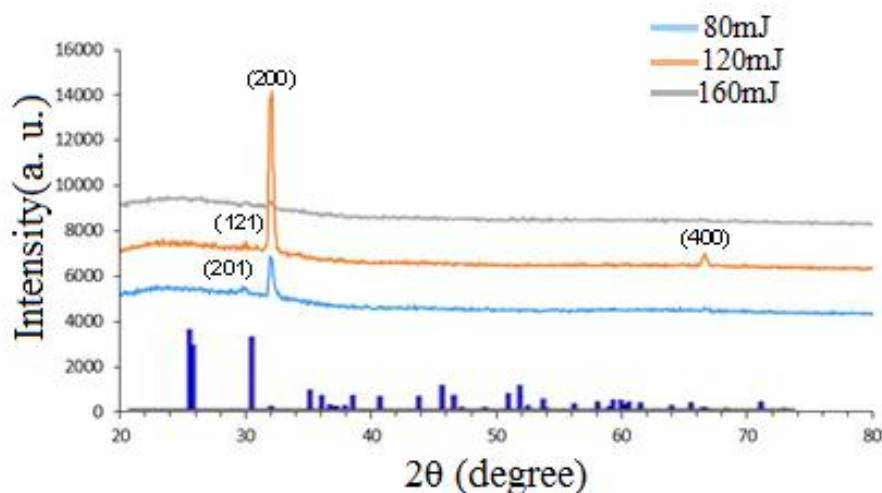
Figure 5: XRD spectra of the TiO 2 NPs prepared at different laser energy standard XRD peaks positions pattern of Brookite TiO 2 placed on x-axis
