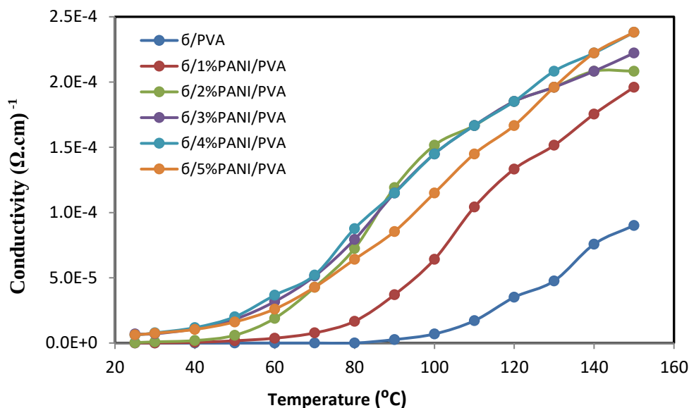
Figure 6: Ionic conductivity as a function of Temperature for PVA before and after PANI addition.
