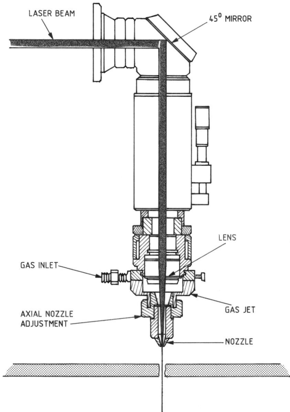
Fig. 4. 2. Laser cutting head showing laser beam path. (after J. Powel 76)
